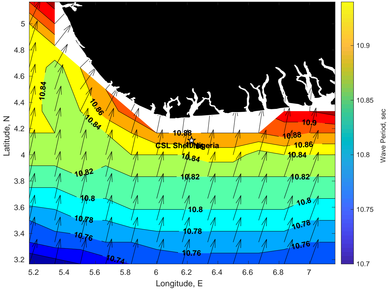
Wave Period (sec) for CSL Shell Nigeria at 26-Jan-2025 09:00:00
