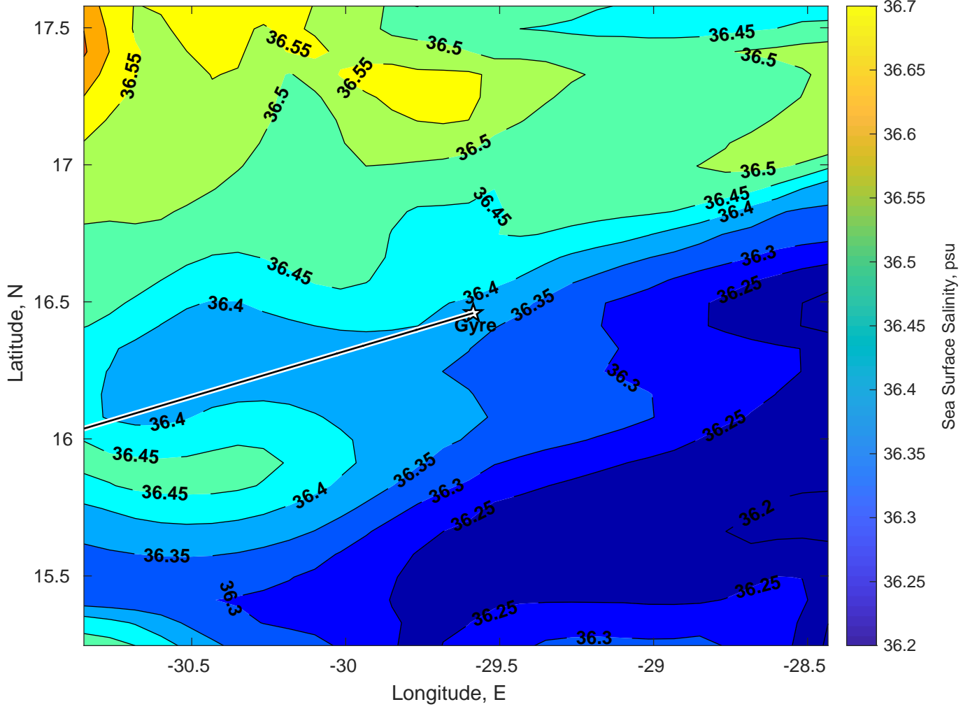
Surface Salinity for Gyre at 25-Jan-2025 00:00:00
