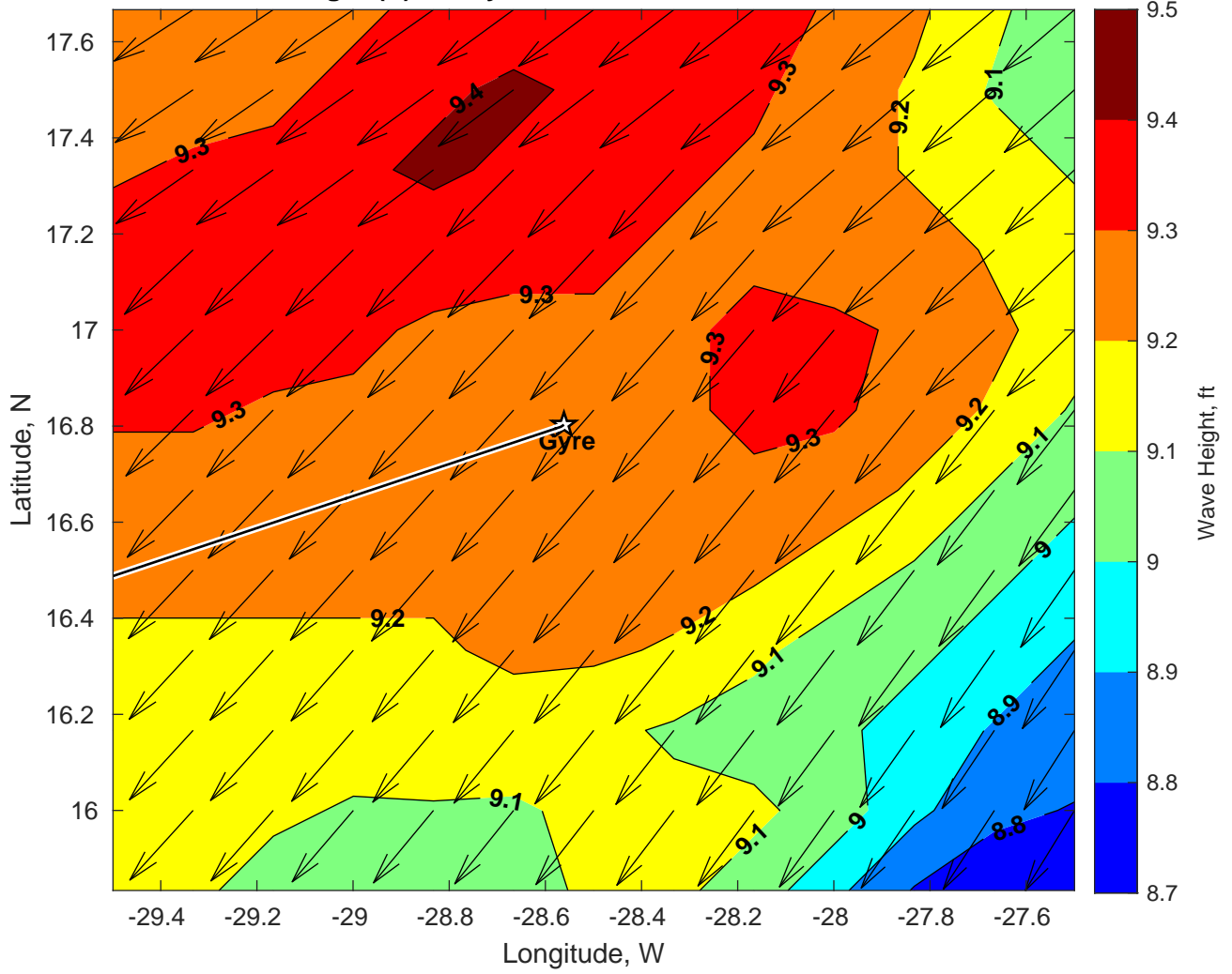
Wave Height (ft) for Gyre at 26-Jan-2025 09:00:00
