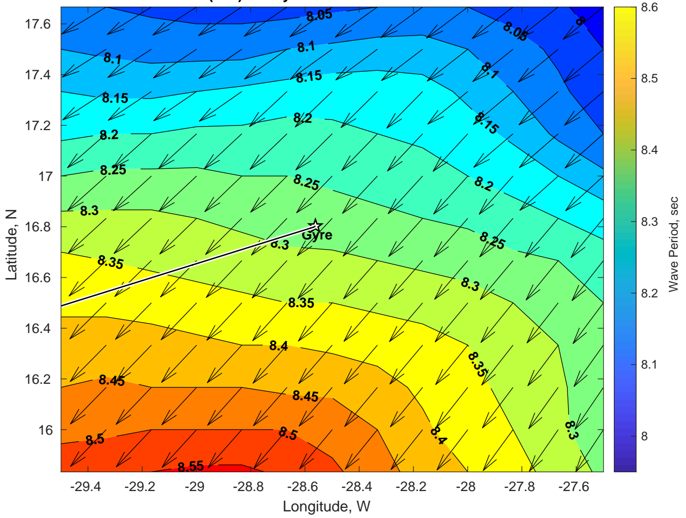
Wave Period (sec) for Gyre at 26-Jan-2025 09:00:00
