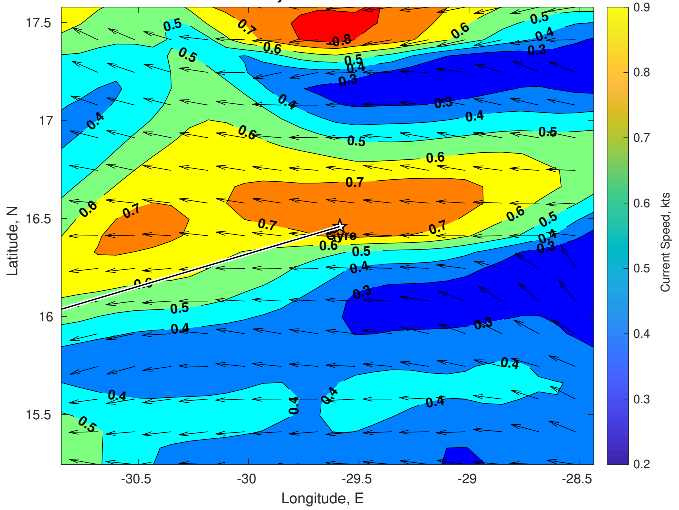
Surface Currents for Gyre at 25-Jan-2025 00:00:00
