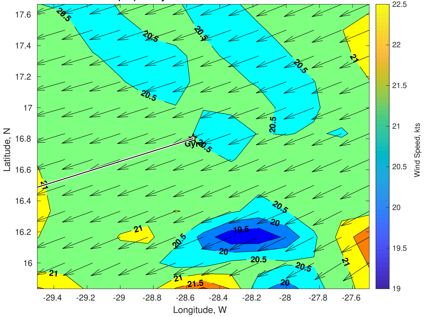
Winds (kts) for Gyre at 26-Jan-2025 09:00:00
