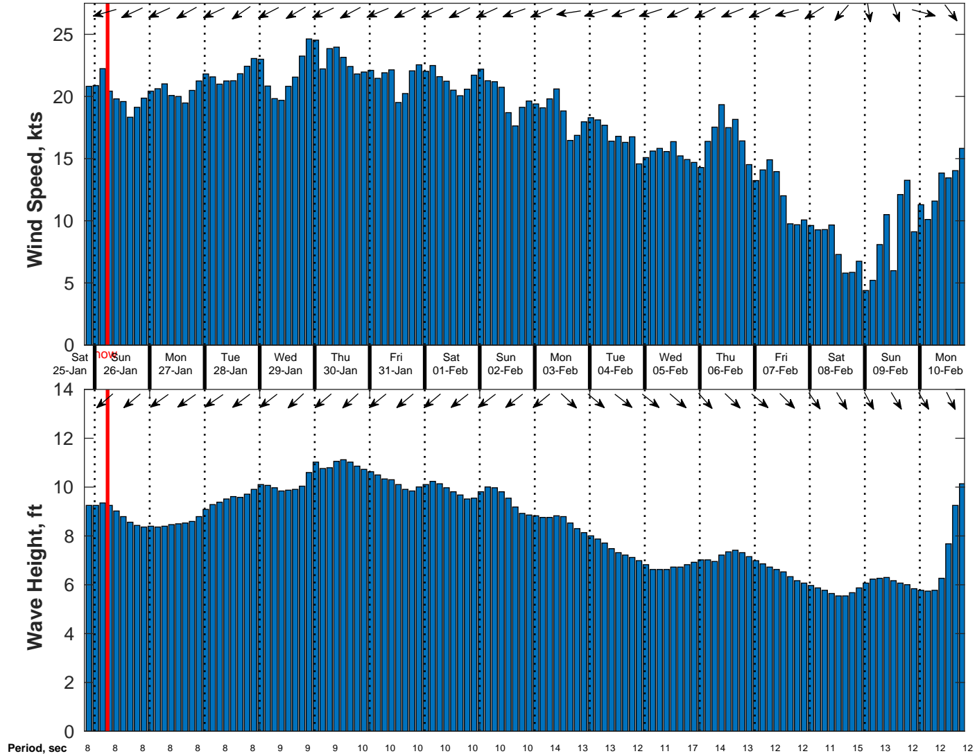
Wind & Wave Forecast for Gyre from 25-Jan-2025 20:00:00 to 10-Feb-2025 20:00:00
