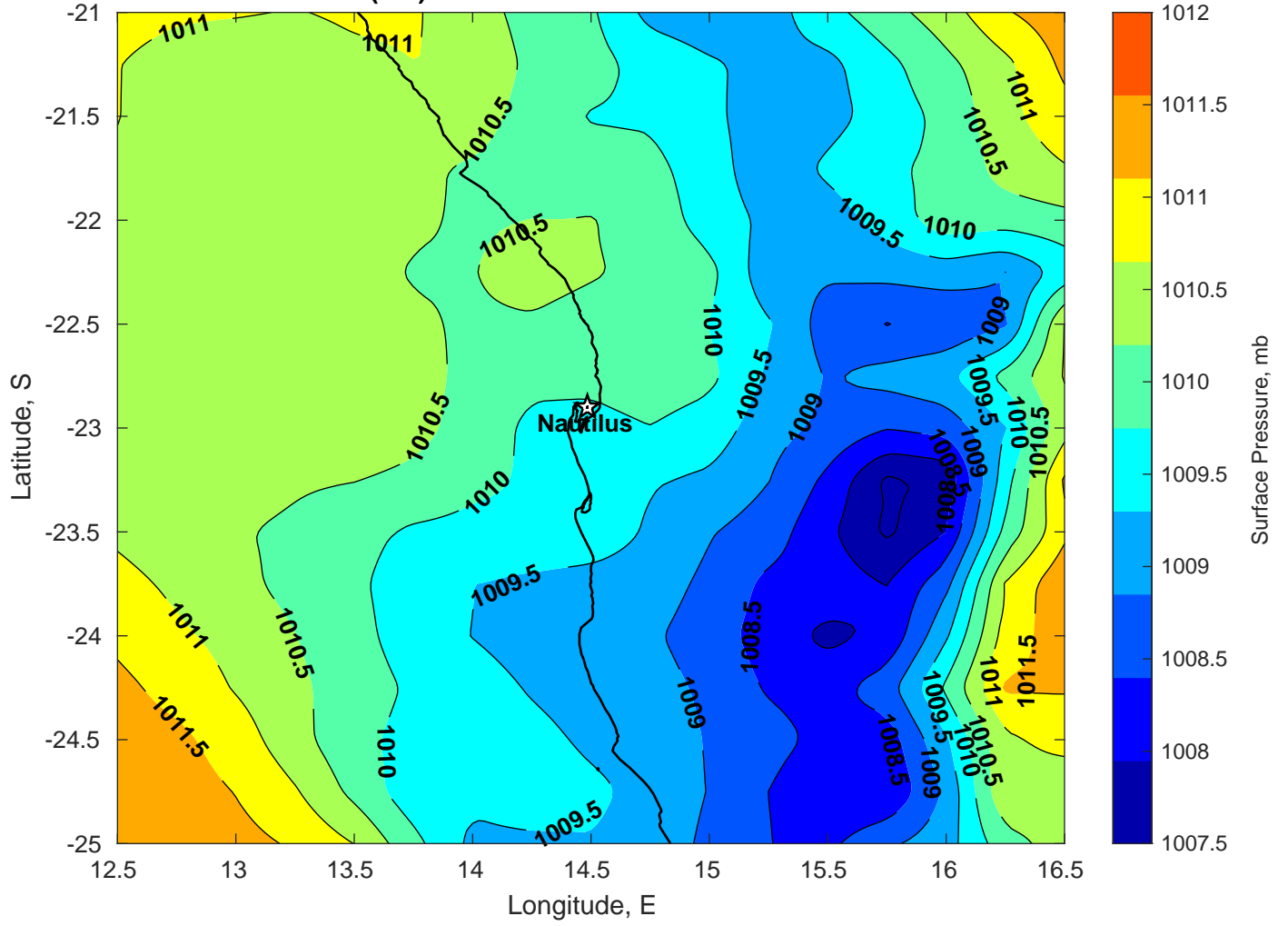
Surface Pressure (mb) for Nautilus at 28-Jan-2025 00:00:00
