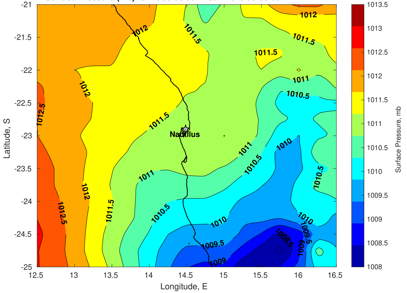
Surface Pressure (mb) for Nautilus at 27-Jan-2025 00:00:00
