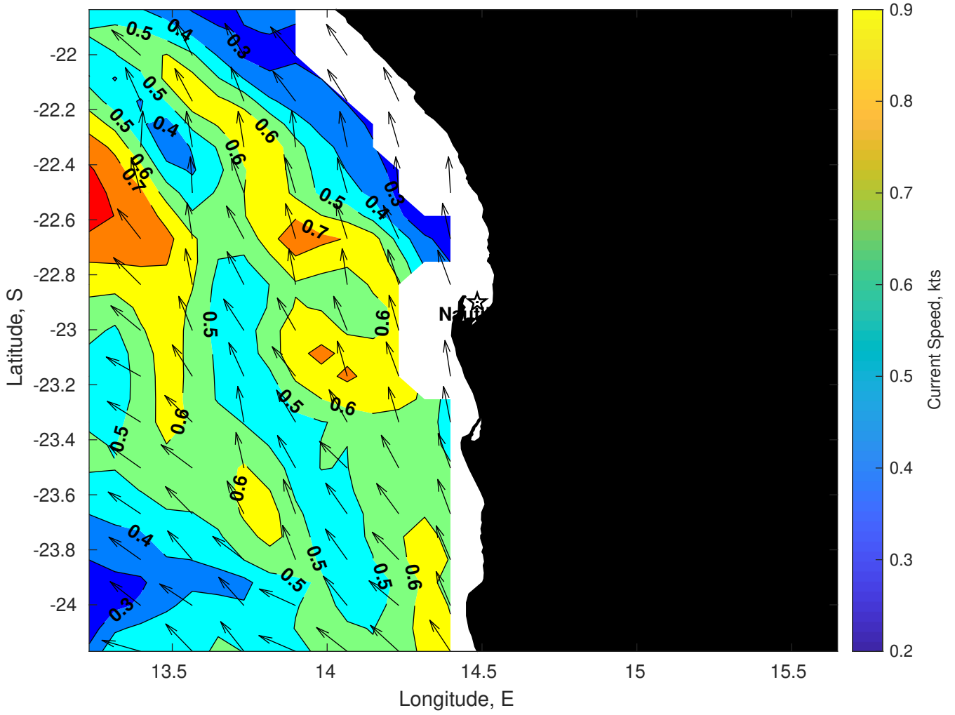
Surface Currents for Nautilus at 25-Jan-2025 00:00:00
