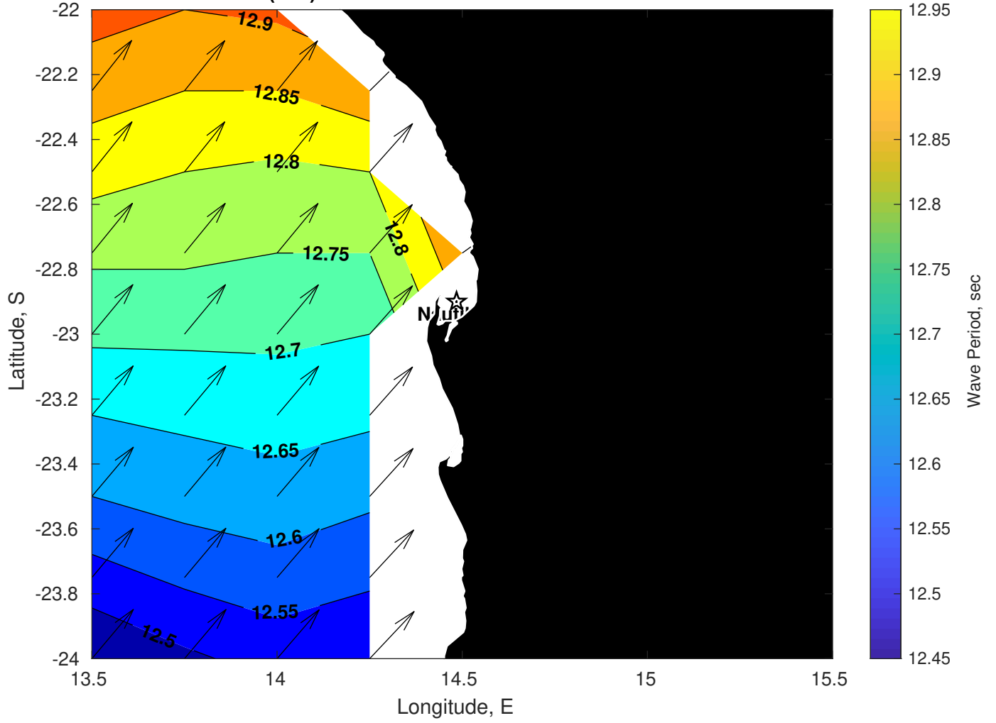
Wave Period (sec) for Nautilus at 26-Jan-2025 09:00:00
