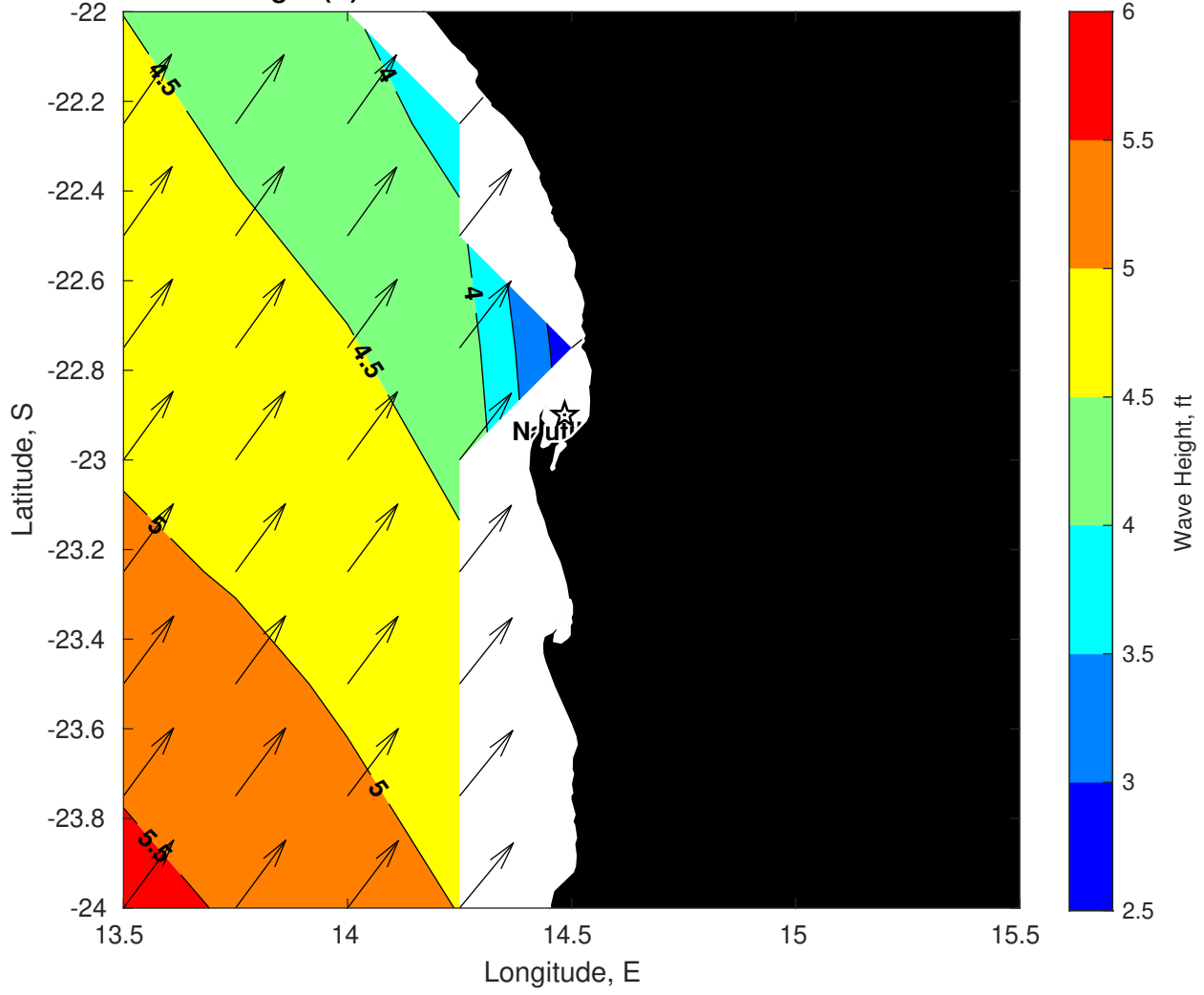
Wave Height (ft) for Nautilus at 26-Jan-2025 09:00:00
