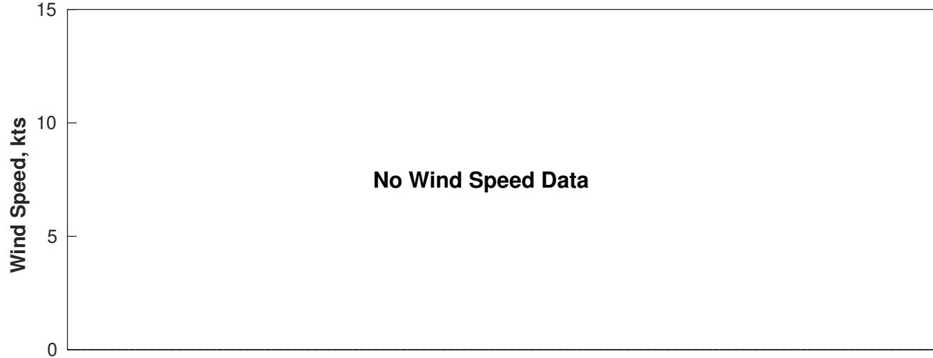
Wind & Wave Forecast for Nautilus from 25-Jan-2025 20:00:00 to 10-Feb-2025 20:00:00
