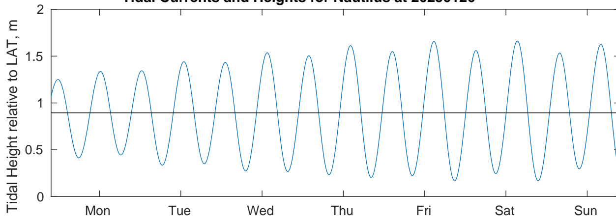
Tidal Currents and Heights for Nautilus at 20250126
