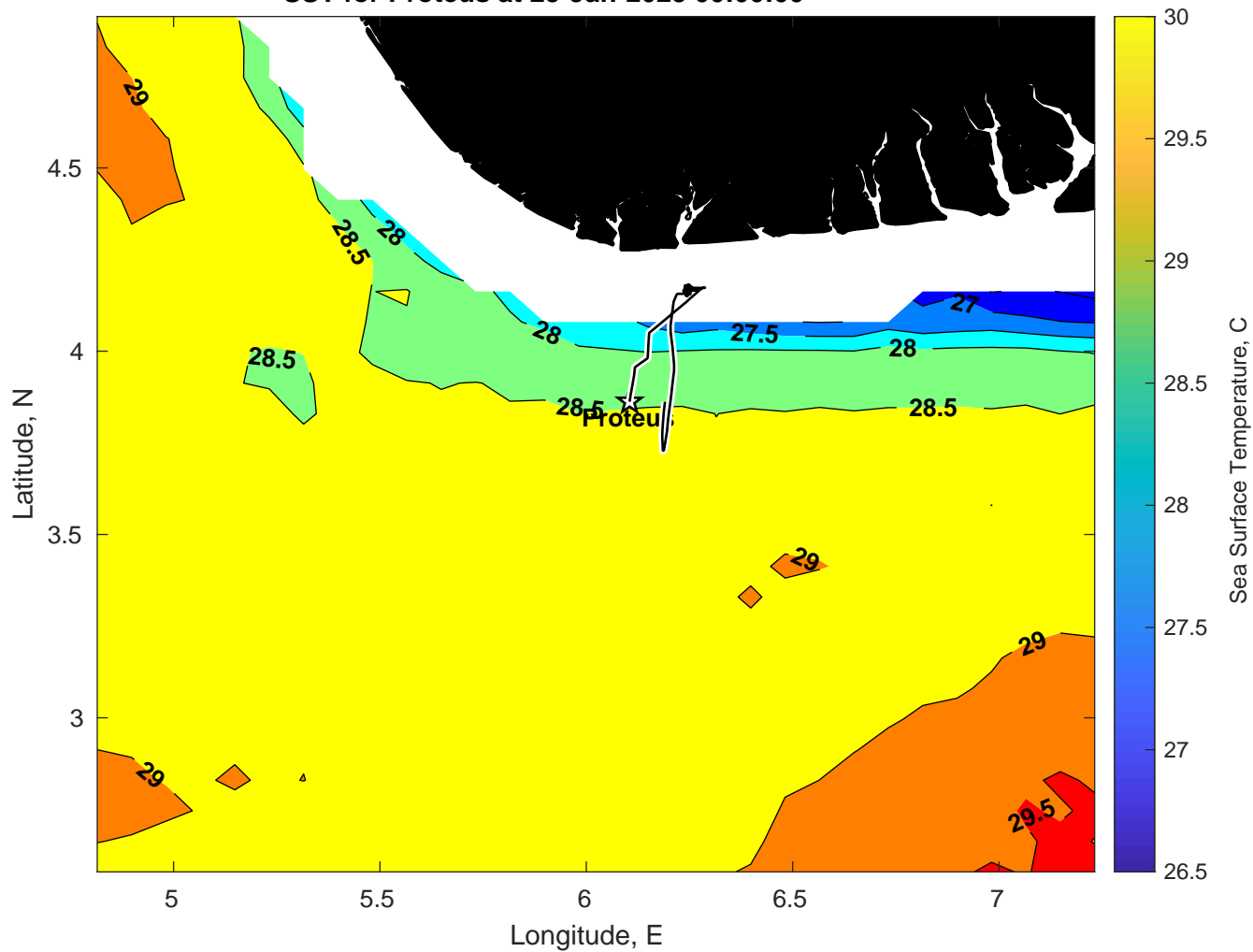
SST for Proteus at 25-Jan-2025 00:00:00
