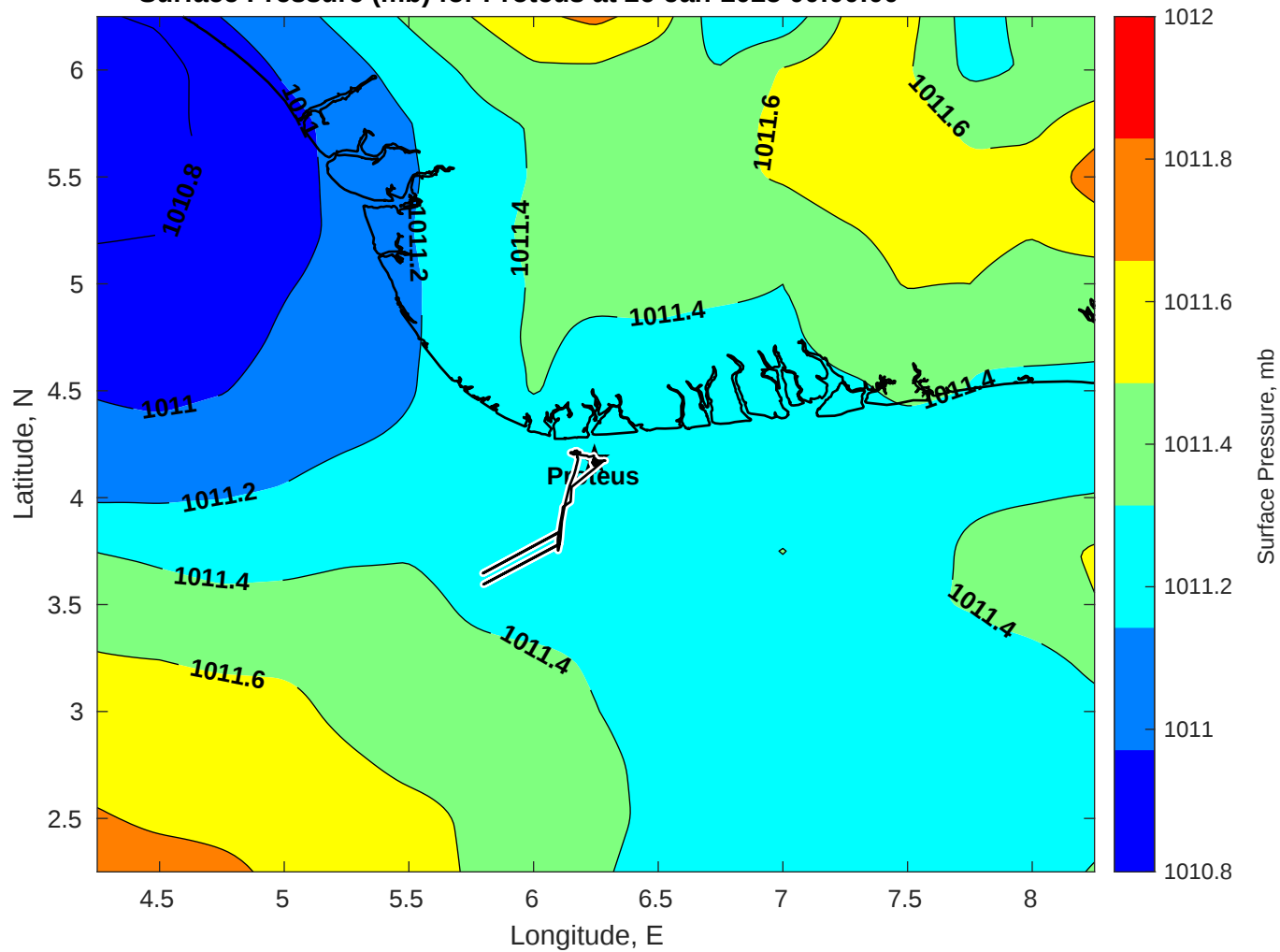
Surface Pressure (mb) for Proteus at 26-Jan-2025 00:00:00
