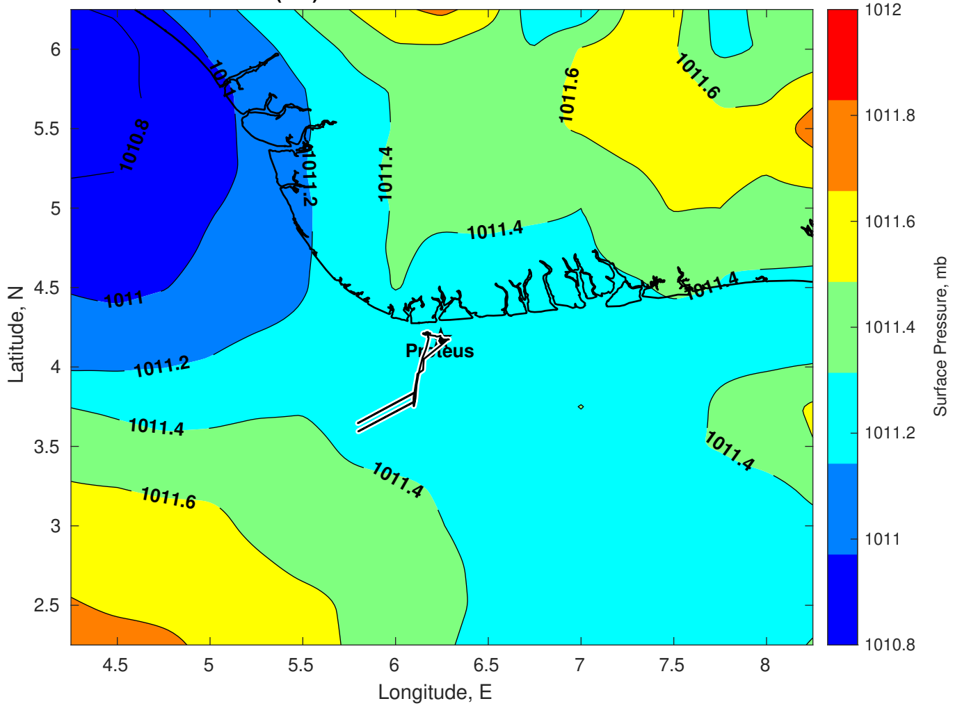
Surface Pressure (mb) for Proteus at 26-Jan-2025 00:00:00
