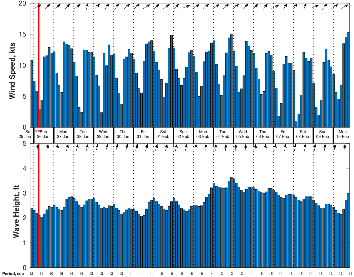
Wind & Wave Forecast for Proteus from 25-Jan-2025 20:00:00 to 10-Feb-2025 20:00:00
