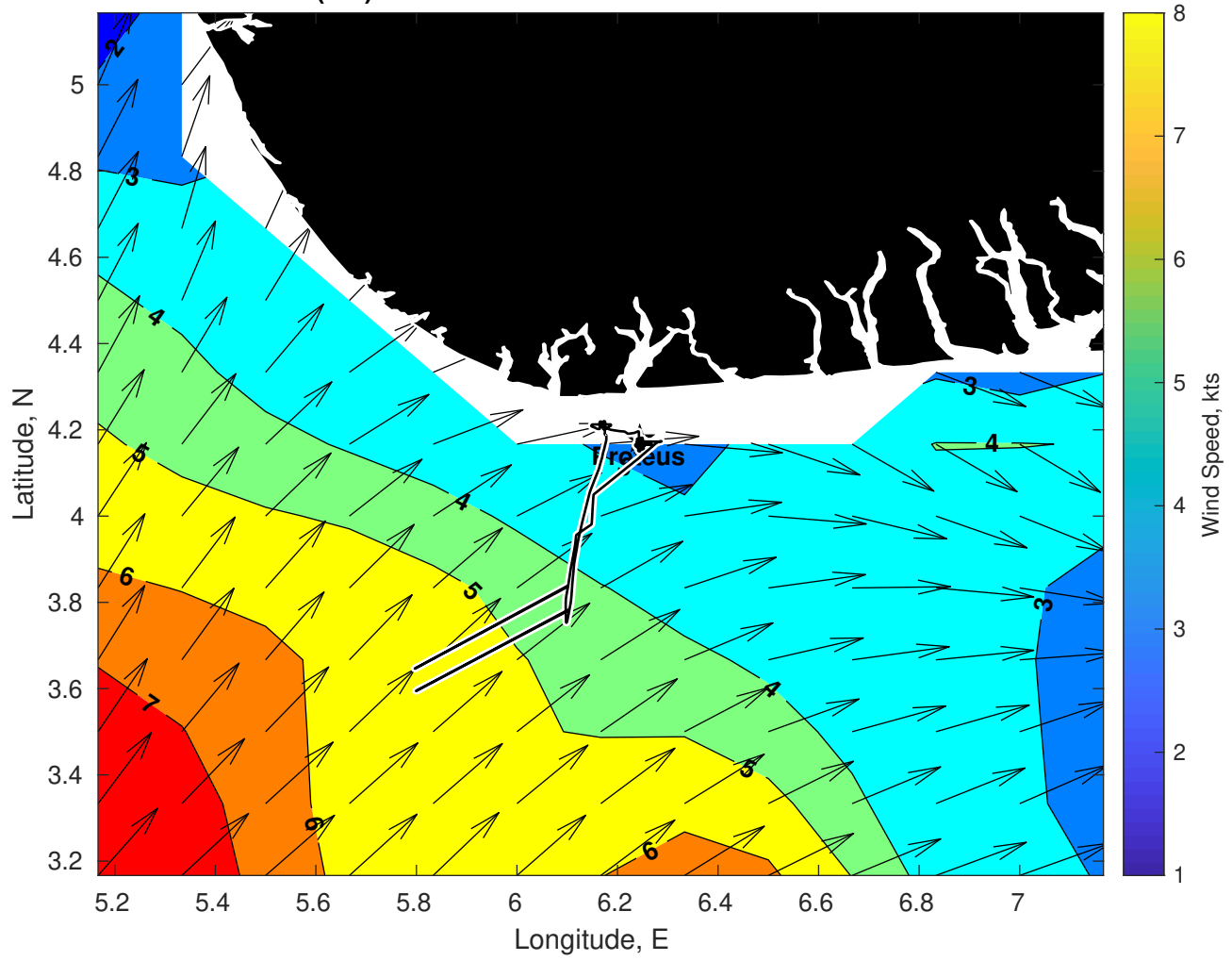
Winds (kts) for Proteus at 26-Jan-2025 09:00:00
