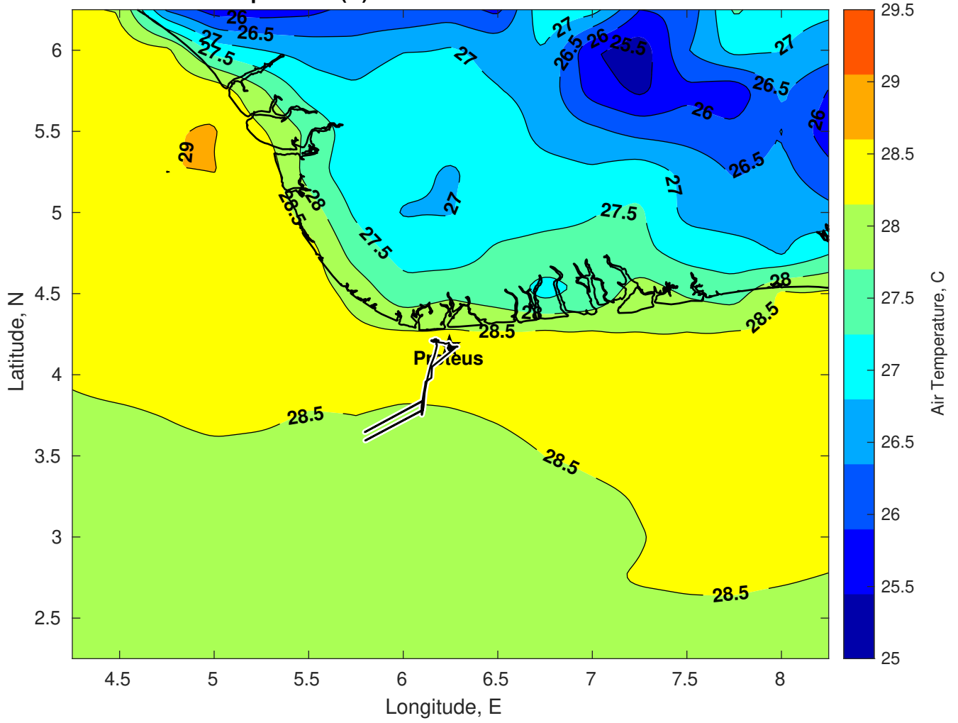
Air Temperature (C) for Proteus at 26-Jan-2025
