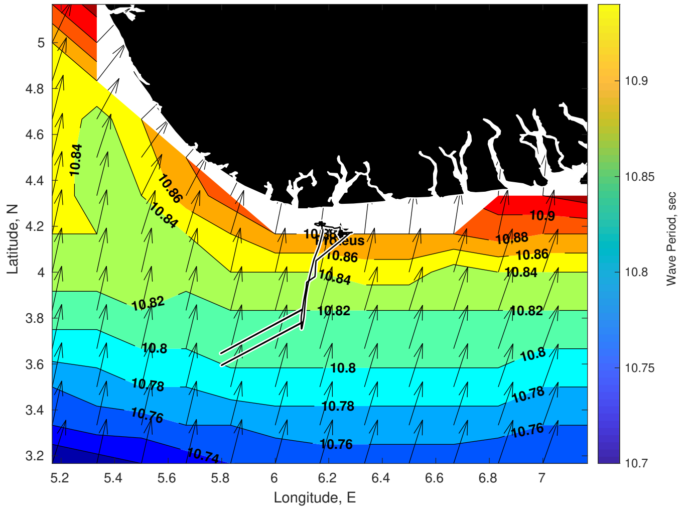
Wave Period (sec) for Proteus at 26-Jan-2025 09:00:00
