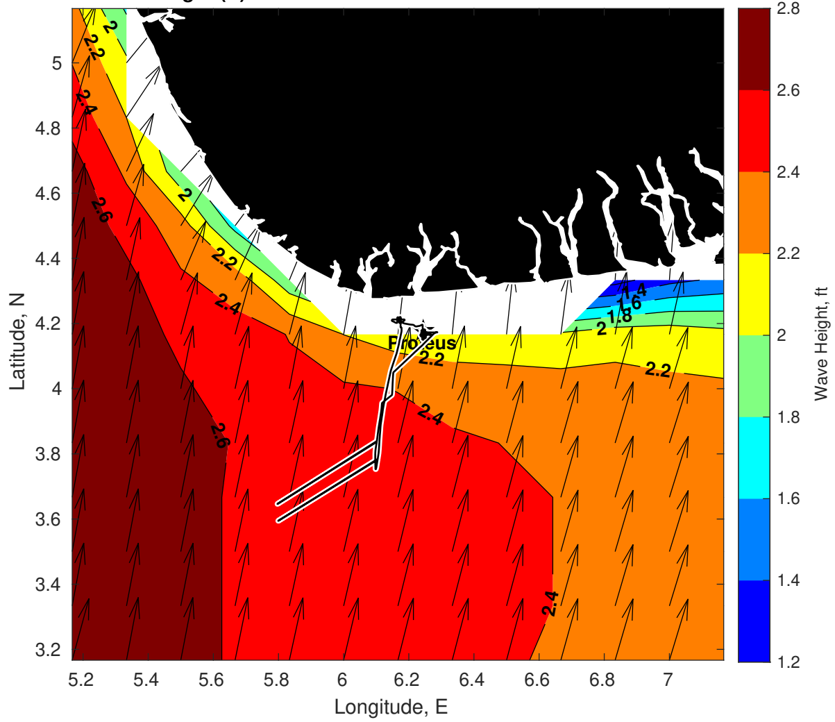
Wave Height (ft) for Proteus at 26-Jan-2025 09:00:00
