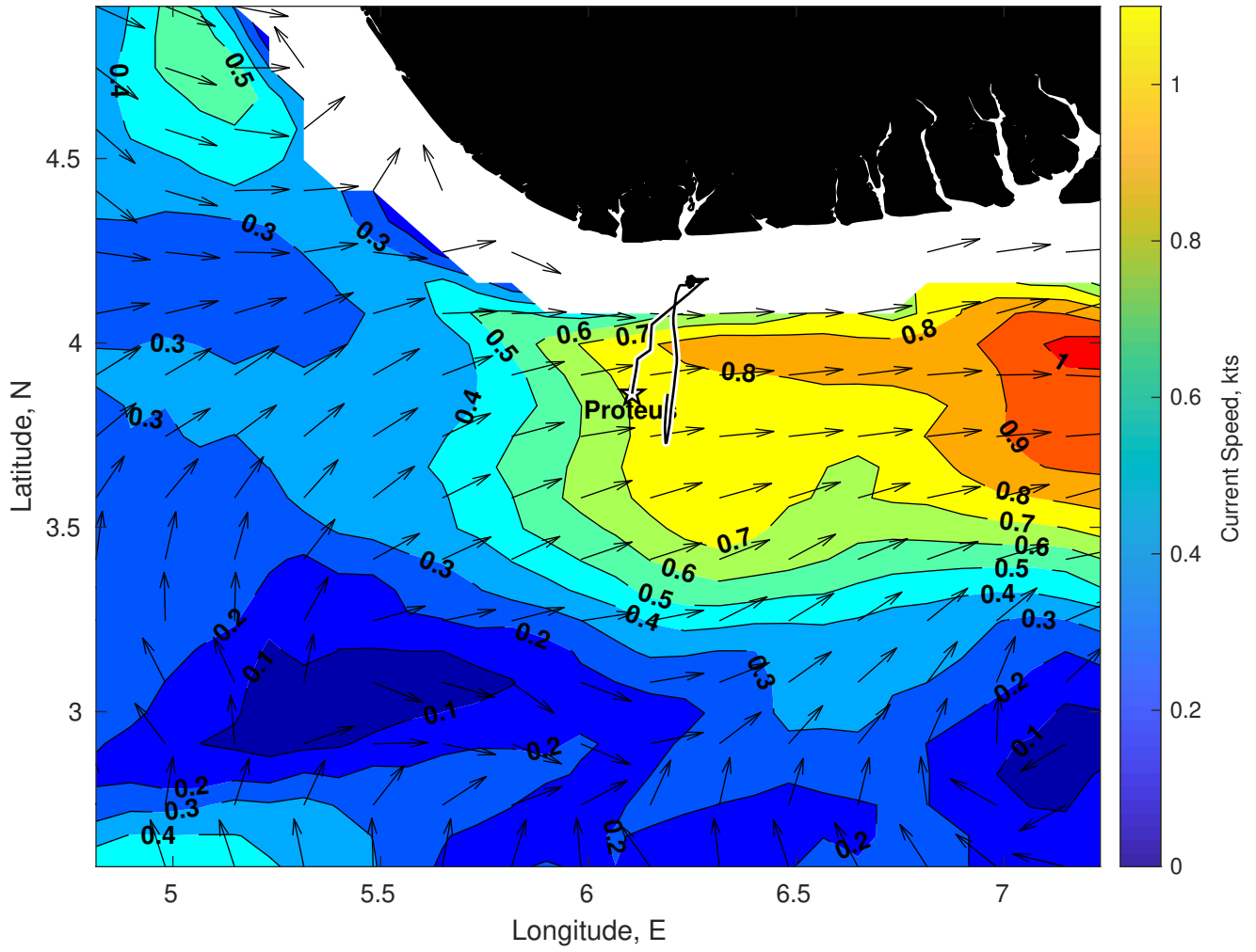
Surface Currents for Proteus at 25-Jan-2025 00:00:00
