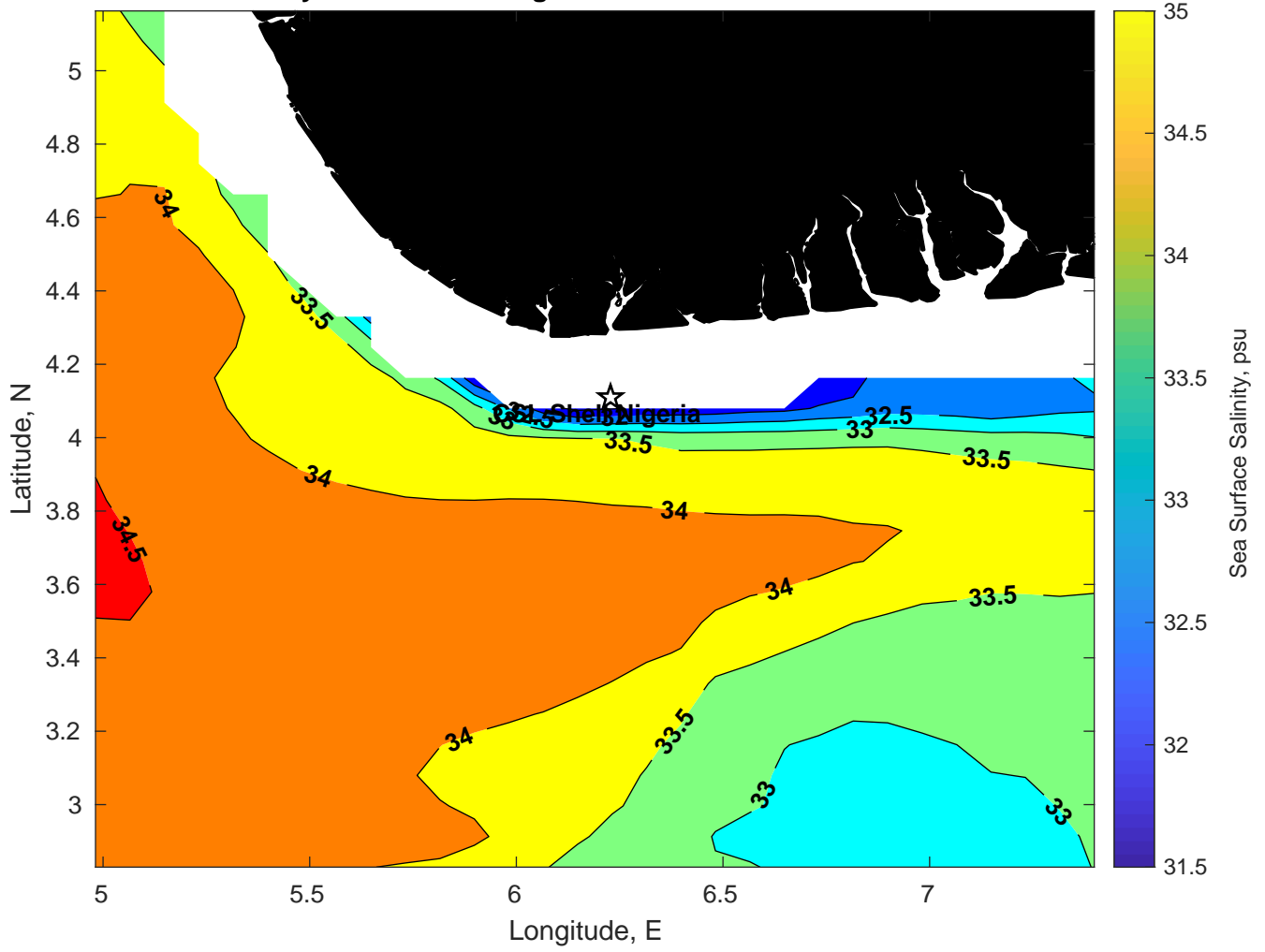
Surface Salinity for CSL Shell Nigeria at 26-Jan-2025 00:00:00
