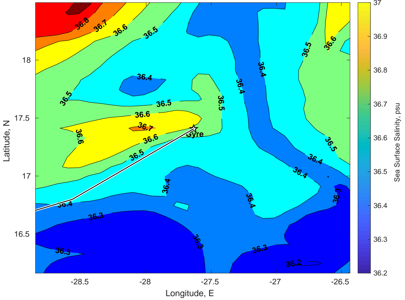
Surface Salinity for Gyre at 26-Jan-2025 00:00:00
