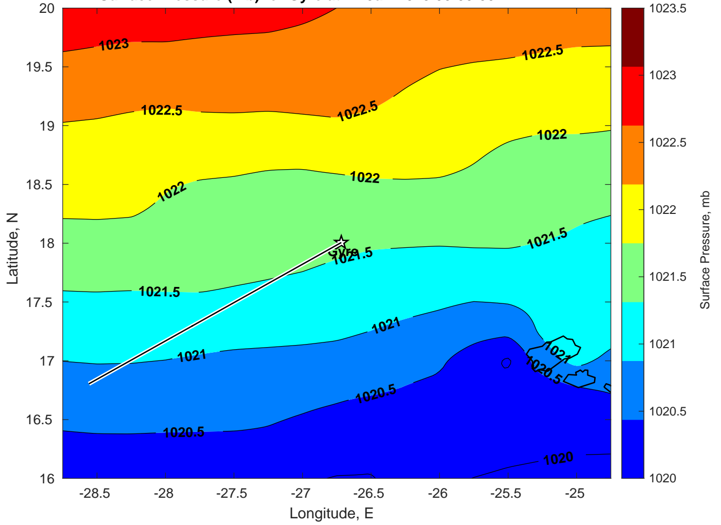
Surface Pressure (mb) for Gyre at 27-Jan-2025 00:00:00
