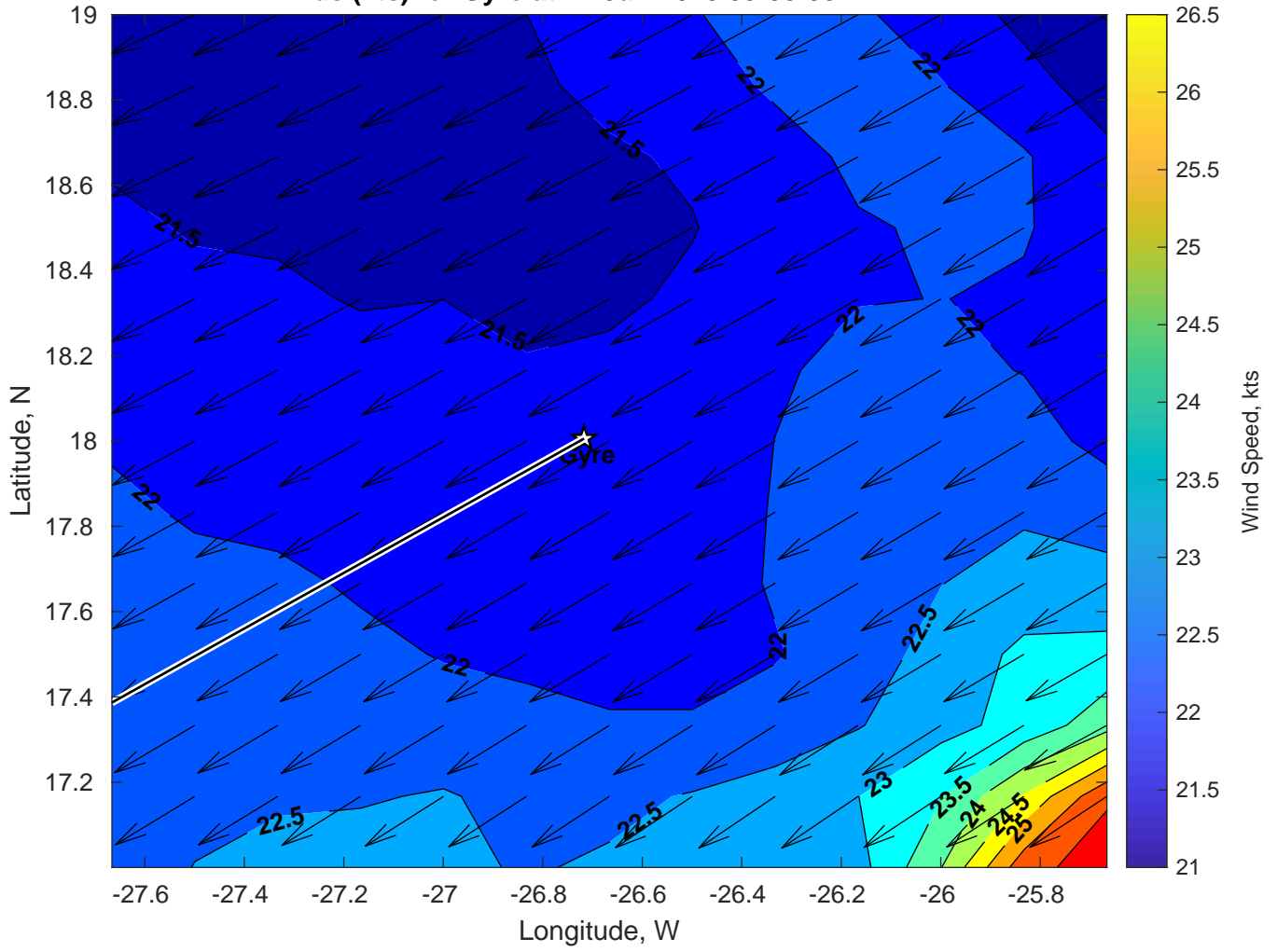
Winds (kts) for Gyre at 27-Jan-2025 09:00:00
