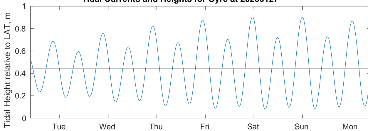
Tidal Currents and Heights for Gyre at 20250127
