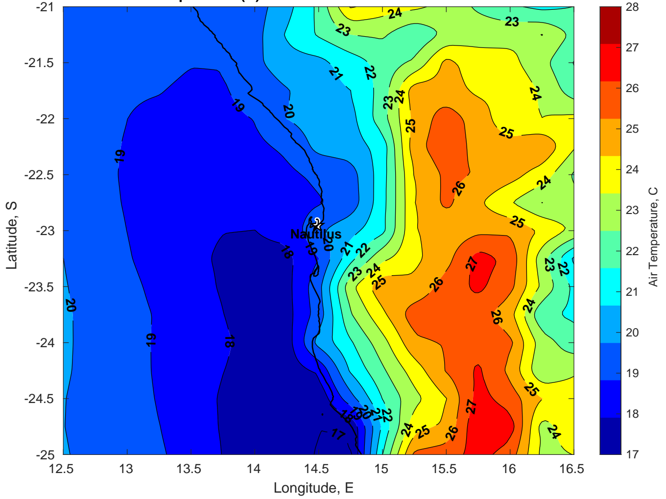
Air Temperature (C) for Nautilus at 27-Jan-2025
