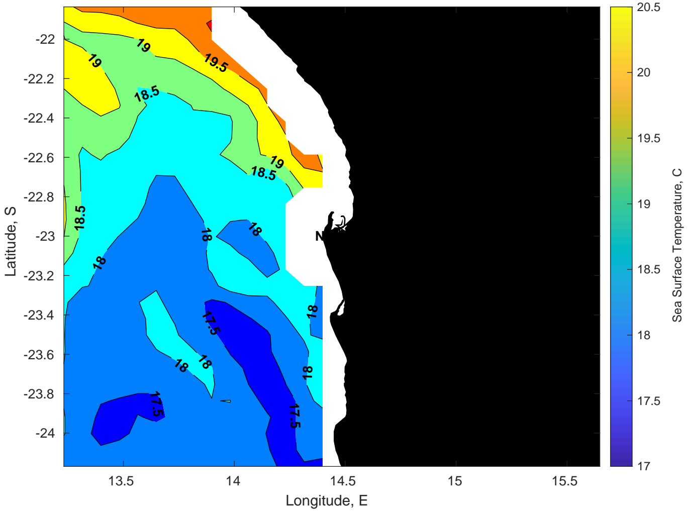
SST for Nautilus at 26-Jan-2025 00:00:00
