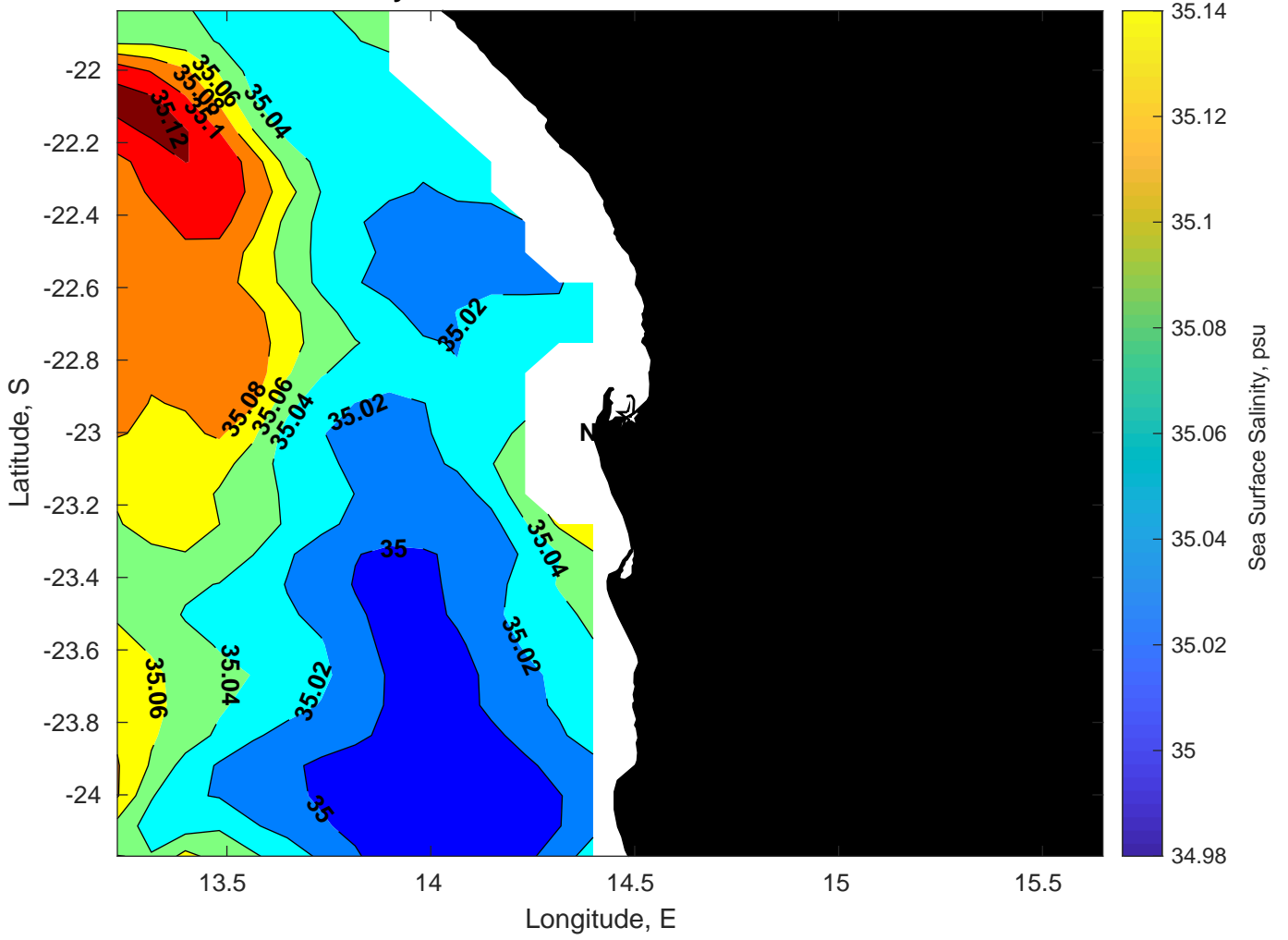
Surface Salinity for Nautilus at 26-Jan-2025 00:00:00
