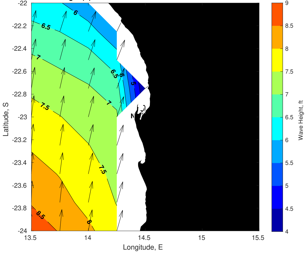
Wave Height (ft) for Nautilus at 27-Jan-2025 09:00:00
