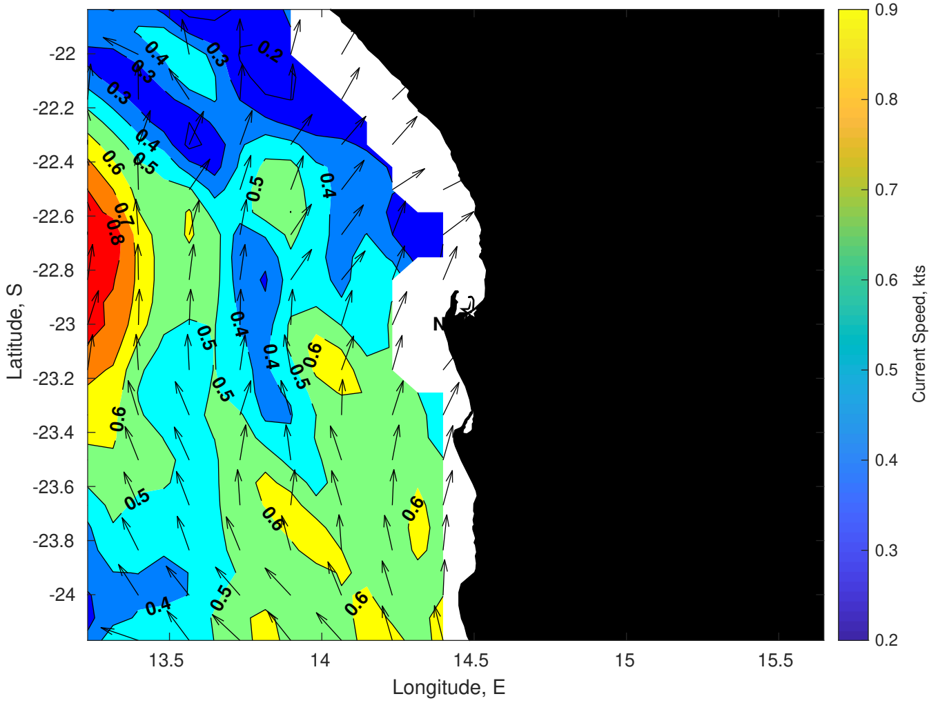
Surface Currents for Nautilus at 26-Jan-2025 00:00:00
