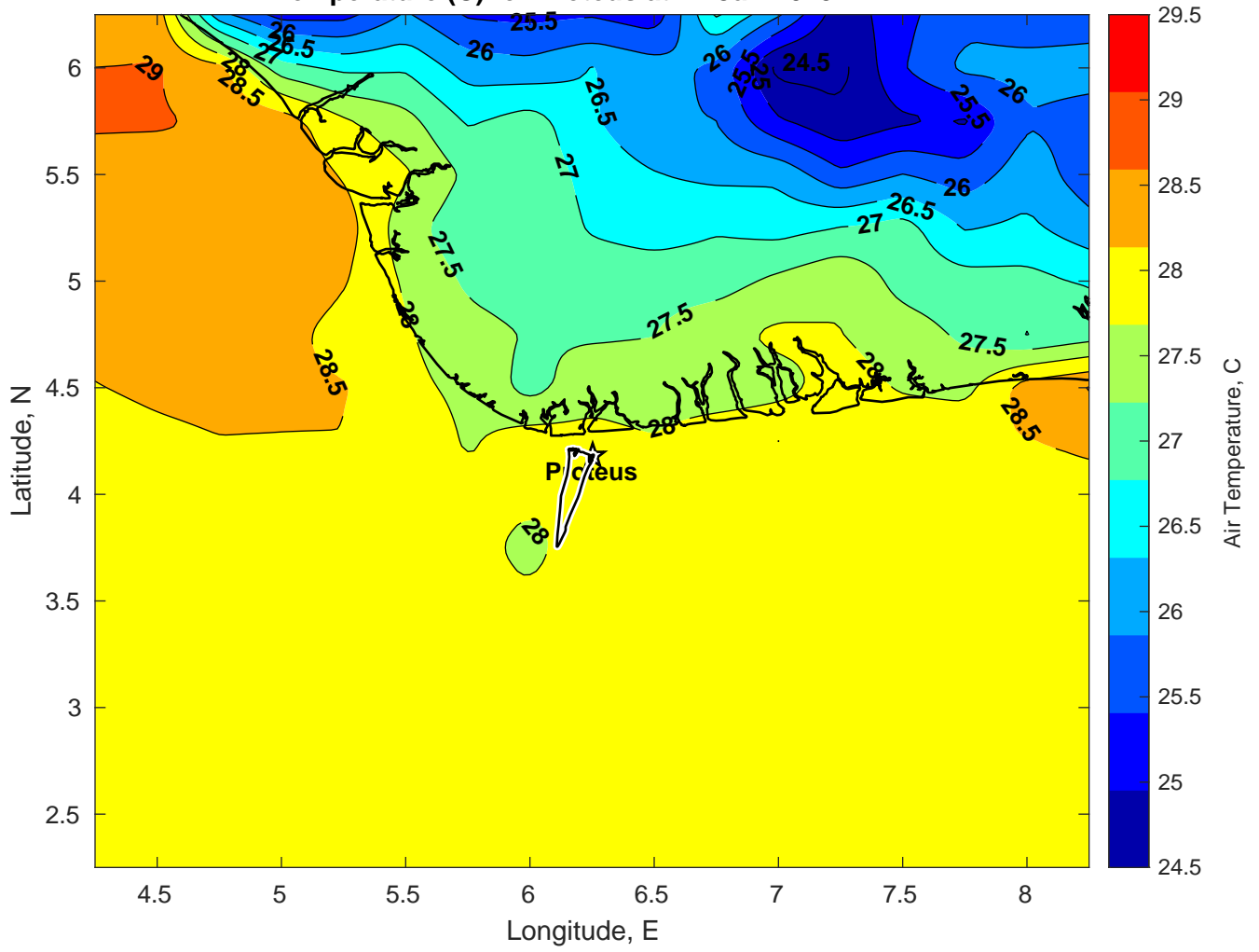
Air Temperature (C) for Proteus at 27-Jan-2025
