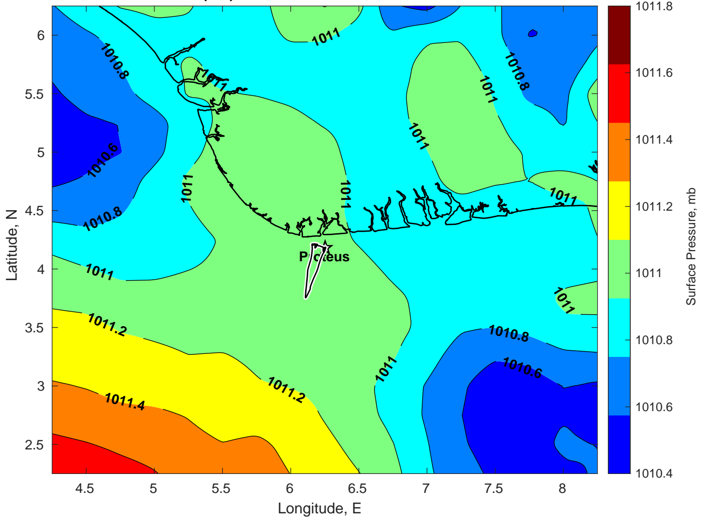
Surface Pressure (mb) for Proteus at 29-Jan-2025 00:00:00
