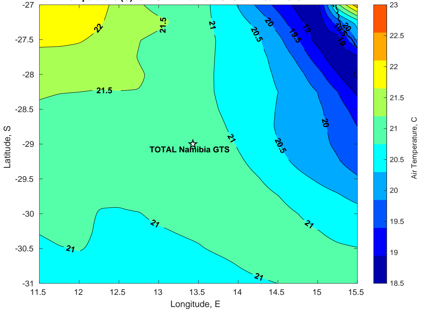
Air Temperature (C) for TOTAL Namibia GTS at 27-Jan-2025
