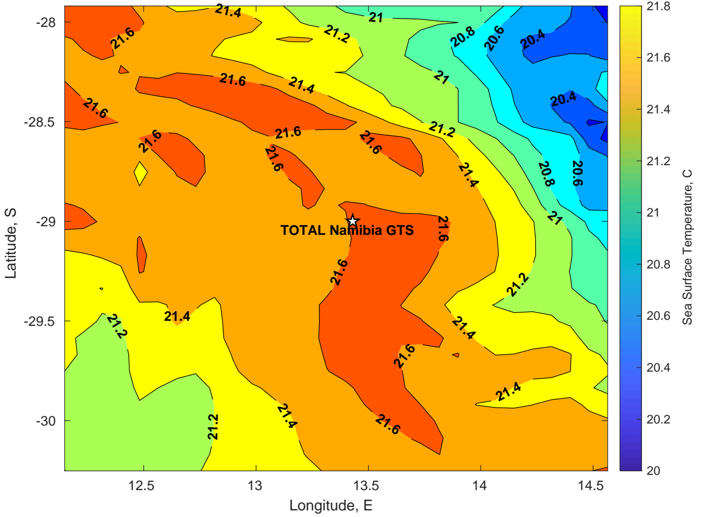
SST for TOTAL Namibia GTS at 26-Jan-2025 00:00:00
