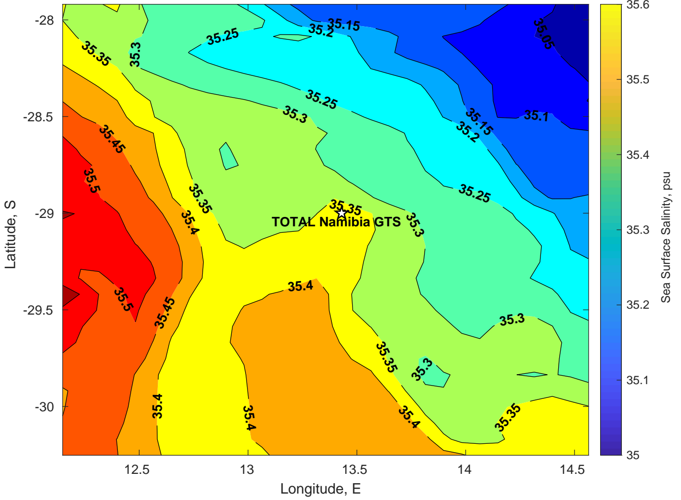
Surface Salinity for TOTAL Namibia GTS at 26-Jan-2025 00:00:00
