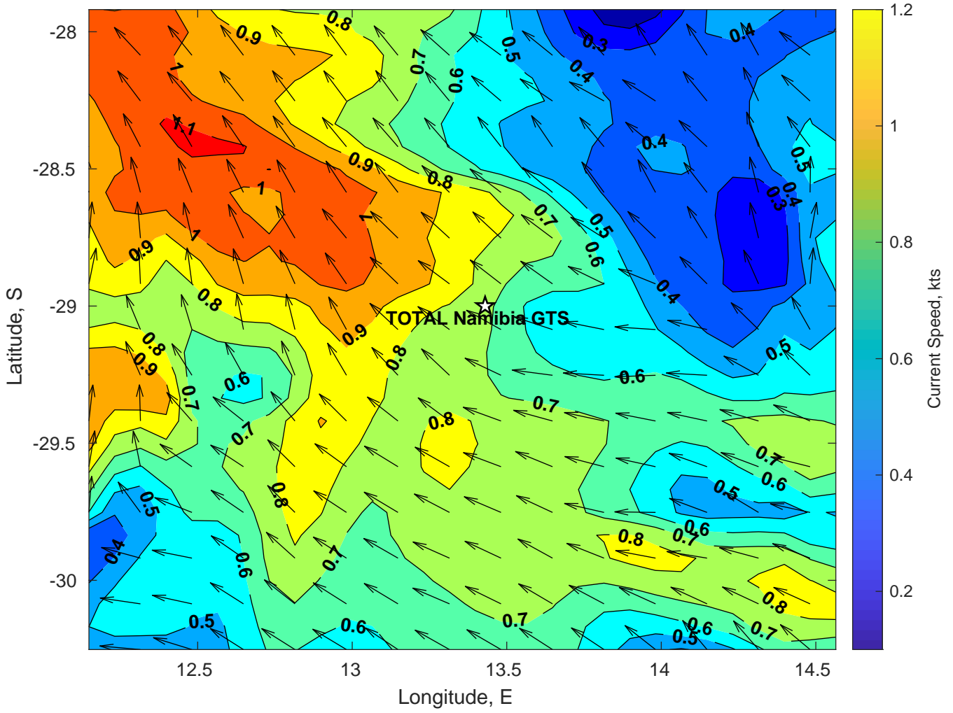
Surface Currents for TOTAL Namibia GTS at 26-Jan-2025 00:00:00
