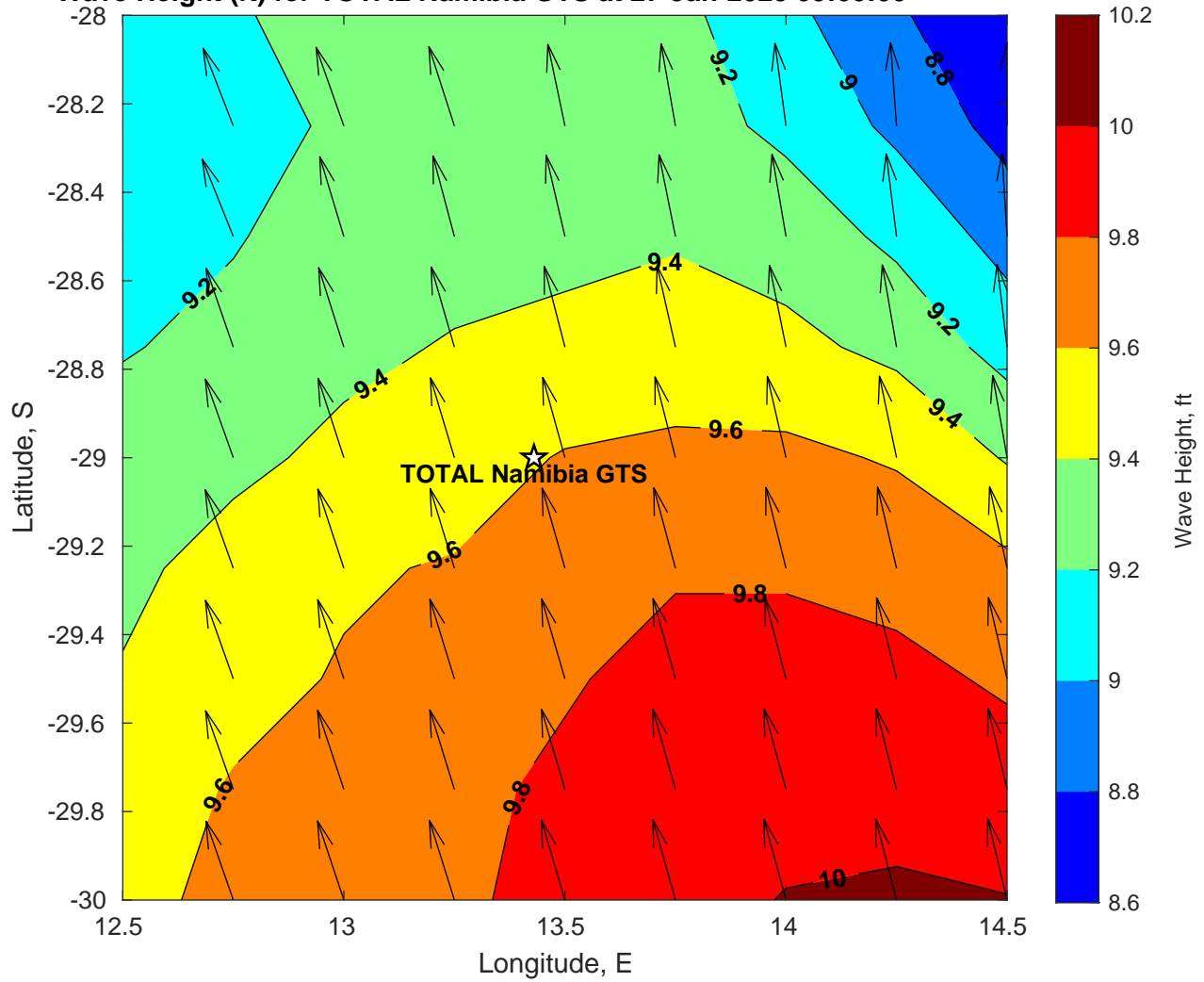
Wave Height (ft) for TOTAL Namibia GTS at 27-Jan-2025 09:00:00
