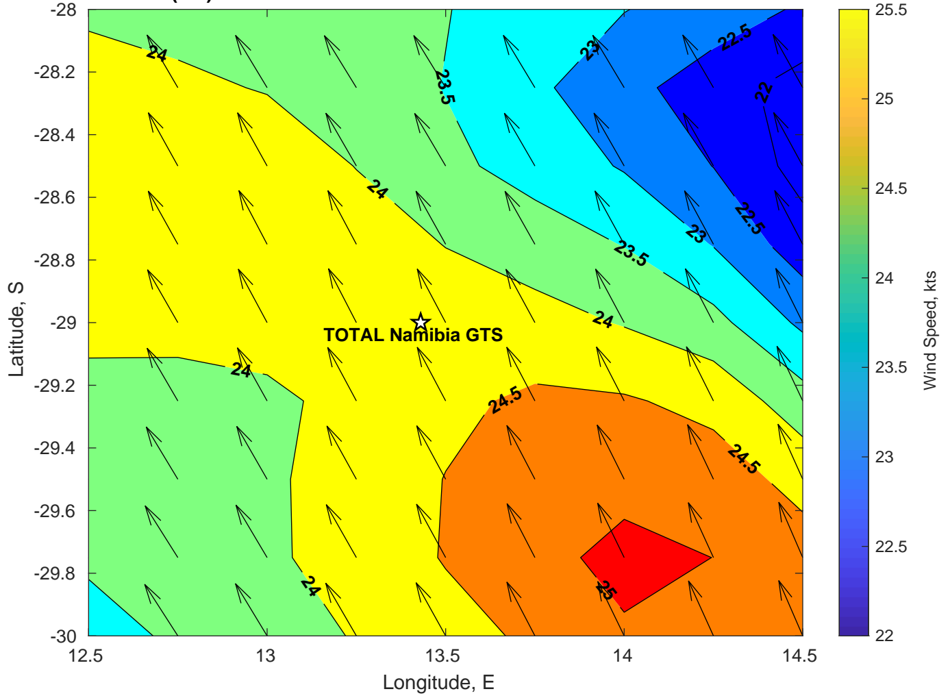
Winds (kts) for TOTAL Namibia GTS at 27-Jan-2025 09:00:00
