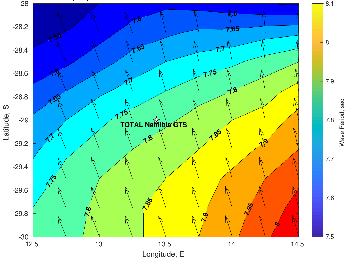
Wave Period (sec) for TOTAL Namibia GTS at 27-Jan-2025 09:00:00
