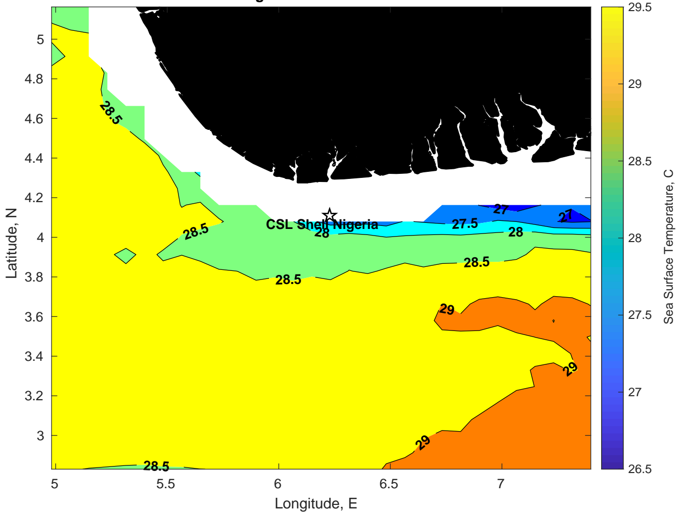
SST for CSL Shell Nigeria at 27-Jan-2025 00:00:00
