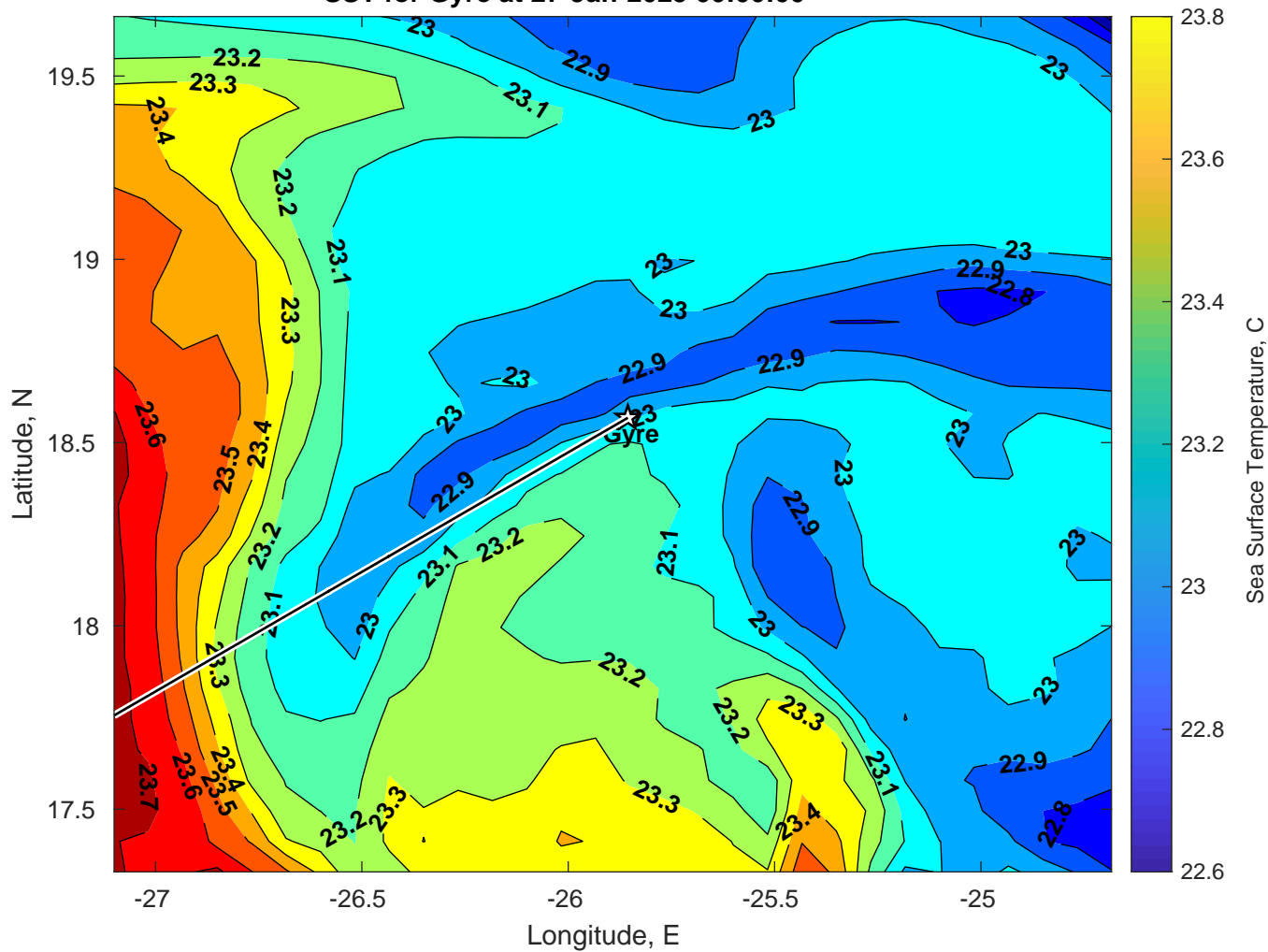
SST for Gyre at 27-Jan-2025 00:00:00
