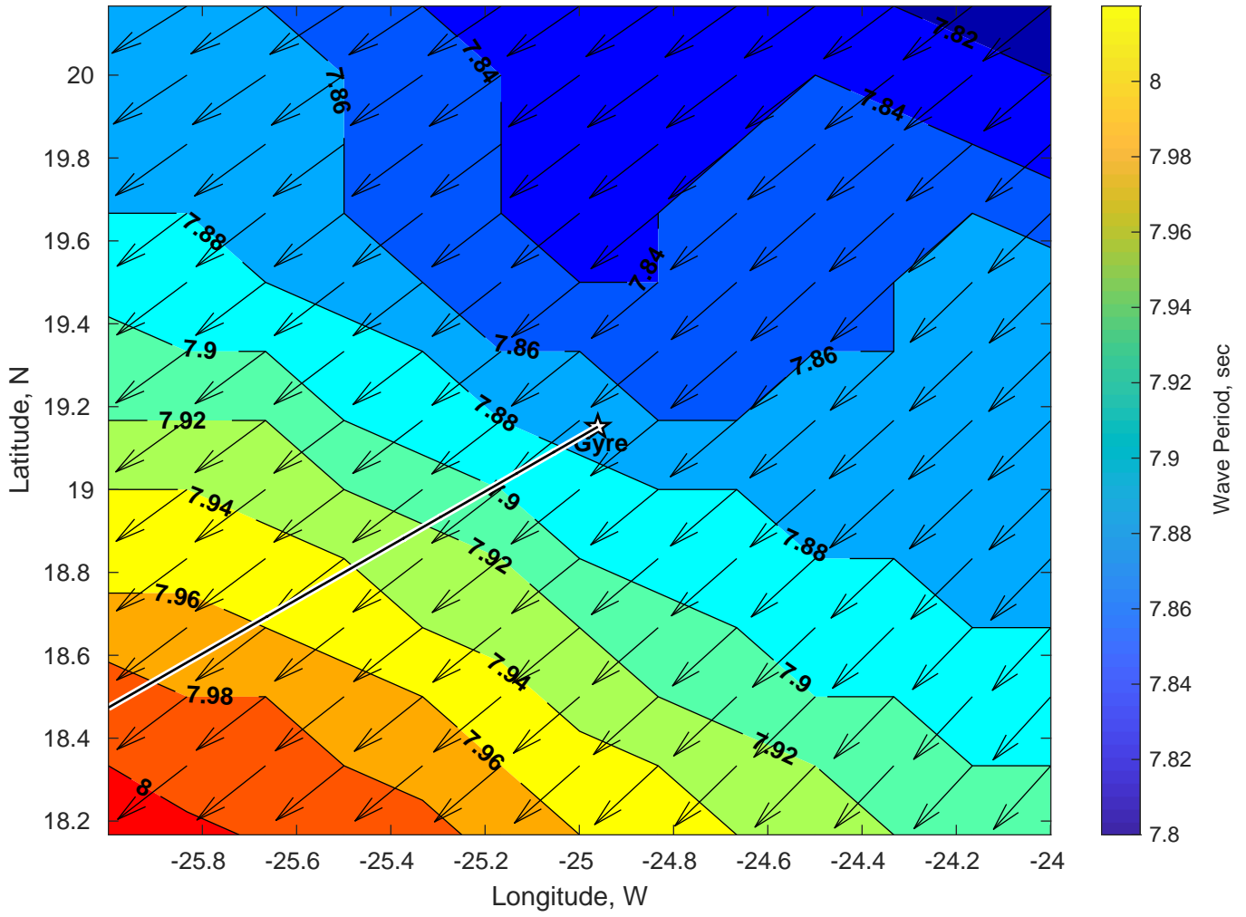
Wave Period (sec) for Gyre at 28-Jan-2025 09:00:00
