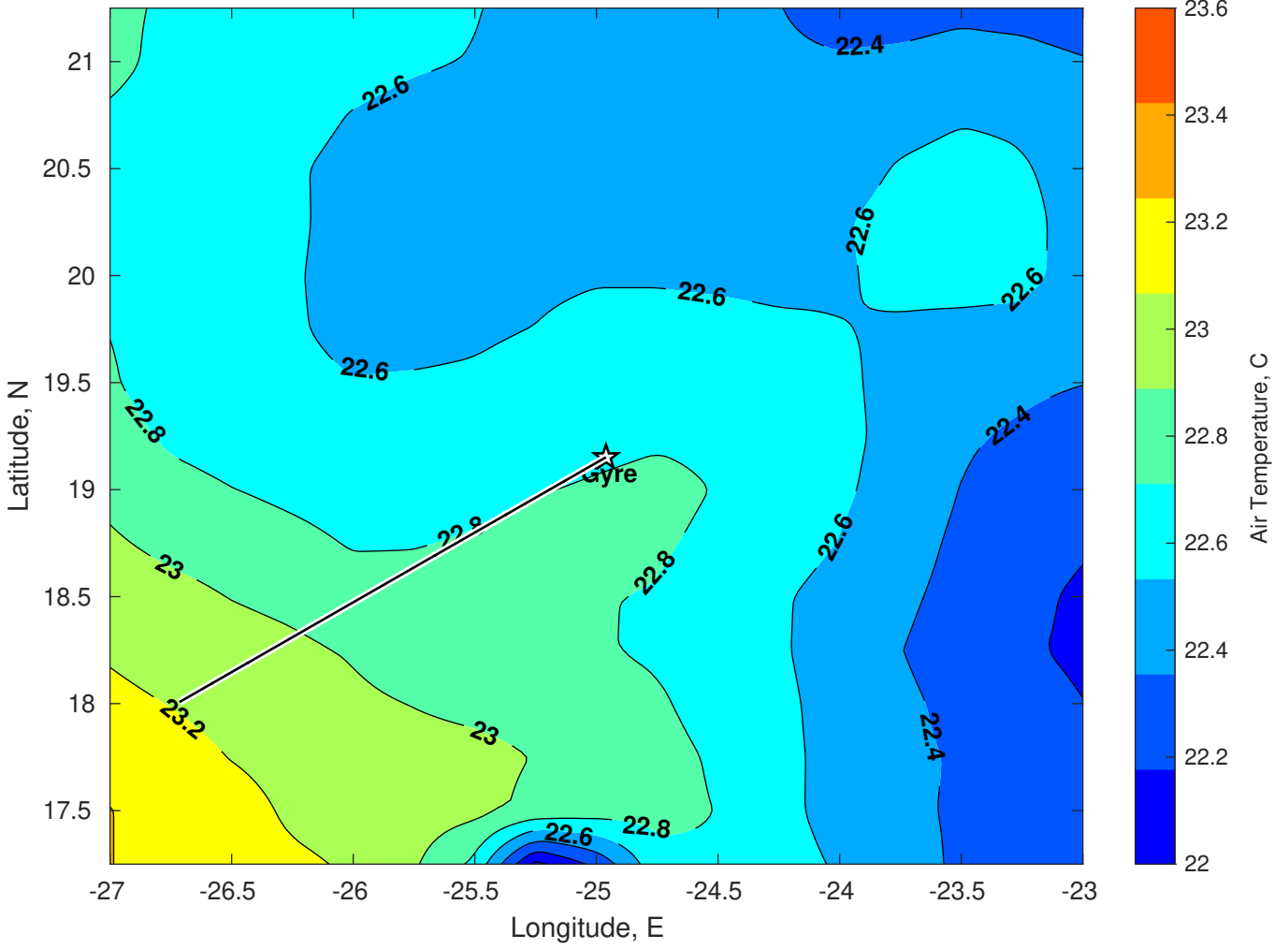
Air Temperature (C) for Gyre at 28-Jan-2025
