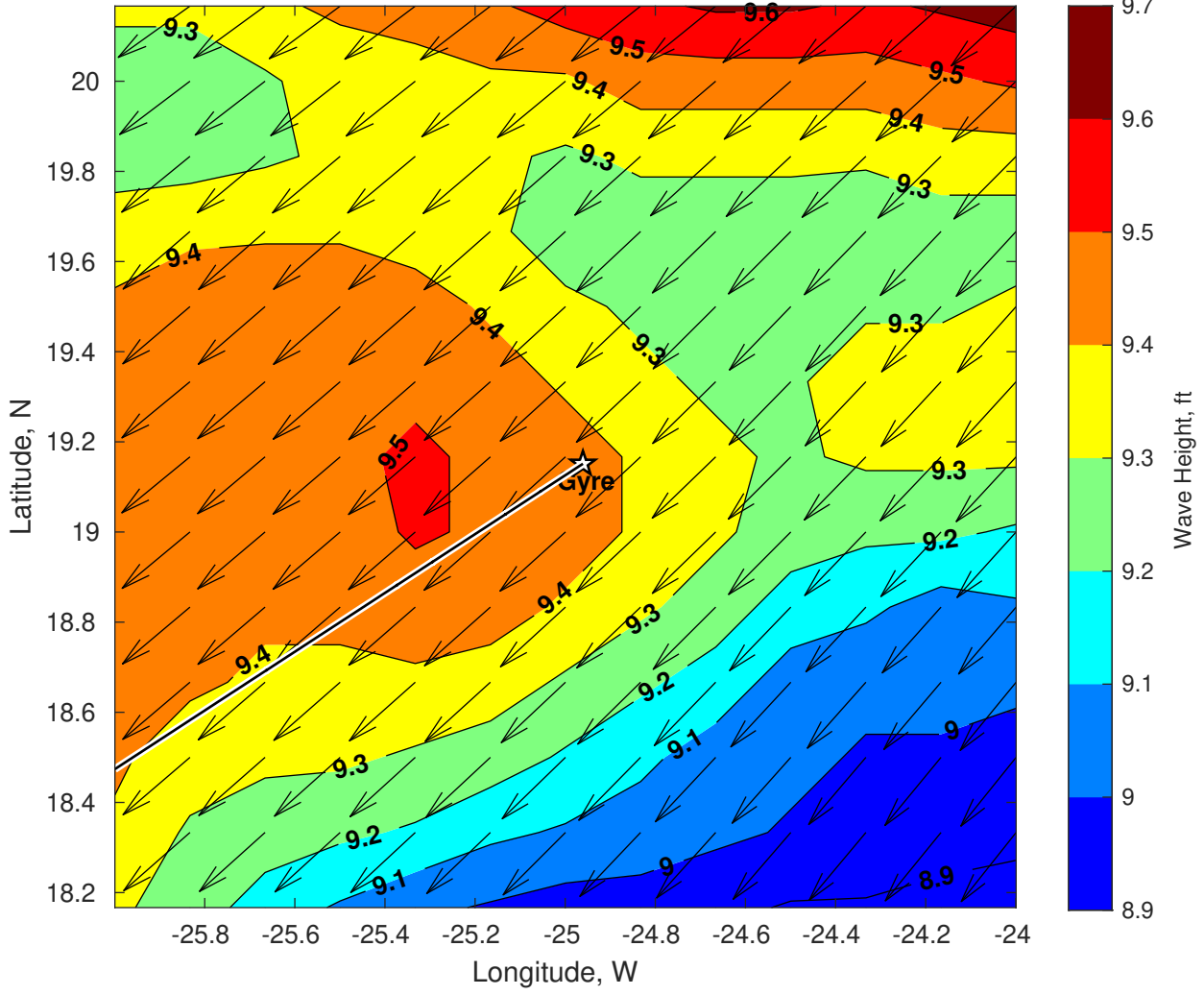
Wave Height (ft) for Gyre at 28-Jan-2025 09:00:00
