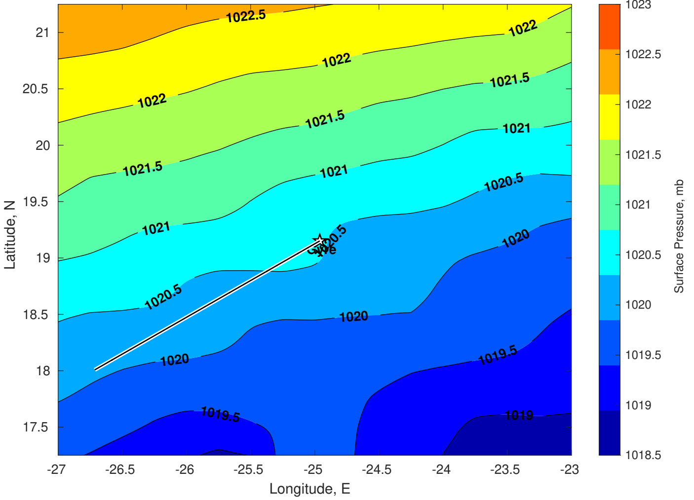
Surface Pressure (mb) for Gyre at 28-Jan-2025 00:00:00
