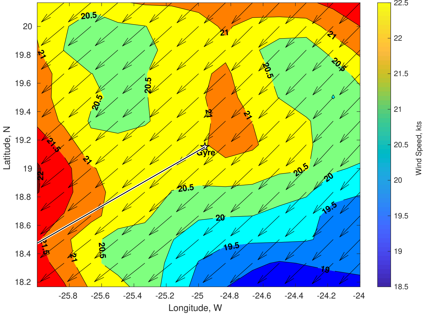
Winds (kts) for Gyre at 28-Jan-2025 09:00:00
