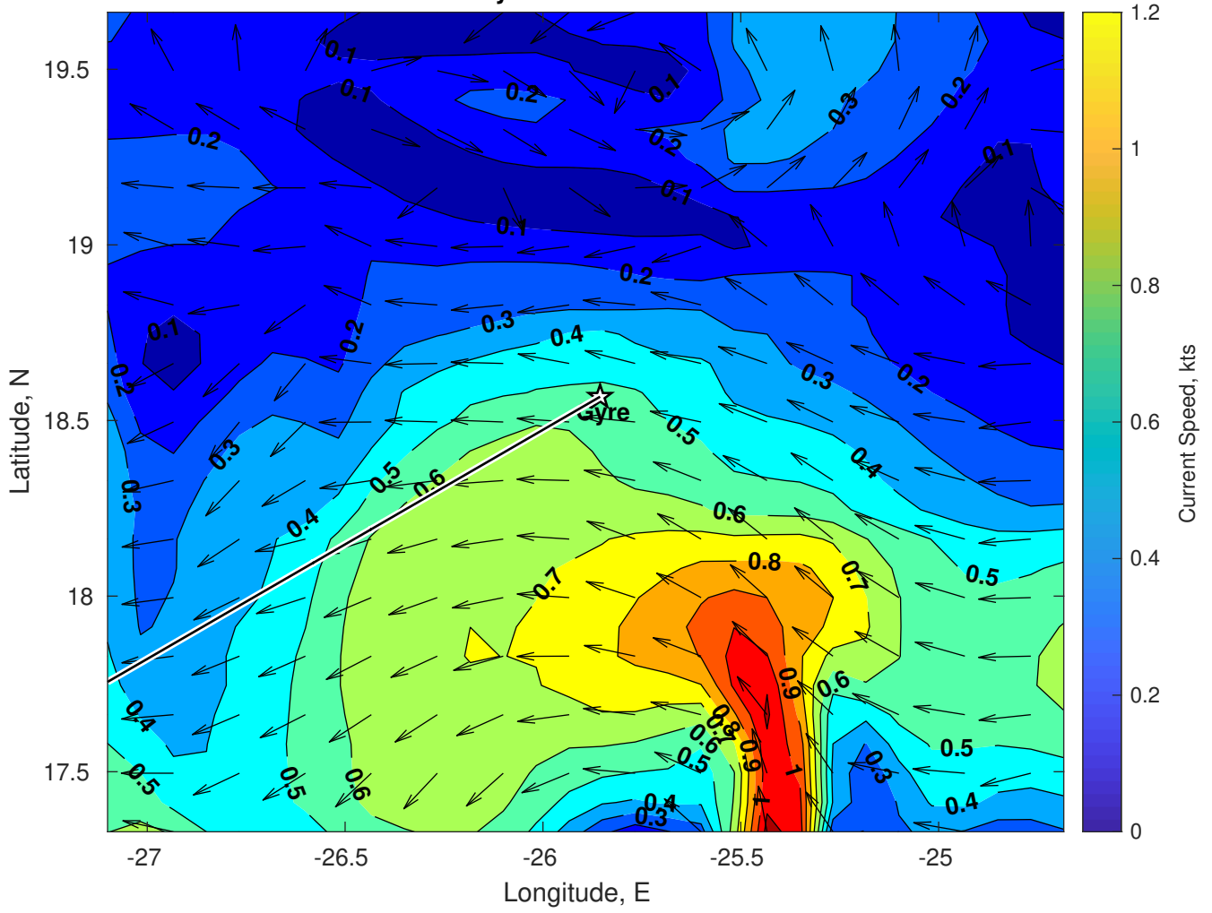
Surface Currents for Gyre at 27-Jan-2025 00:00:00
