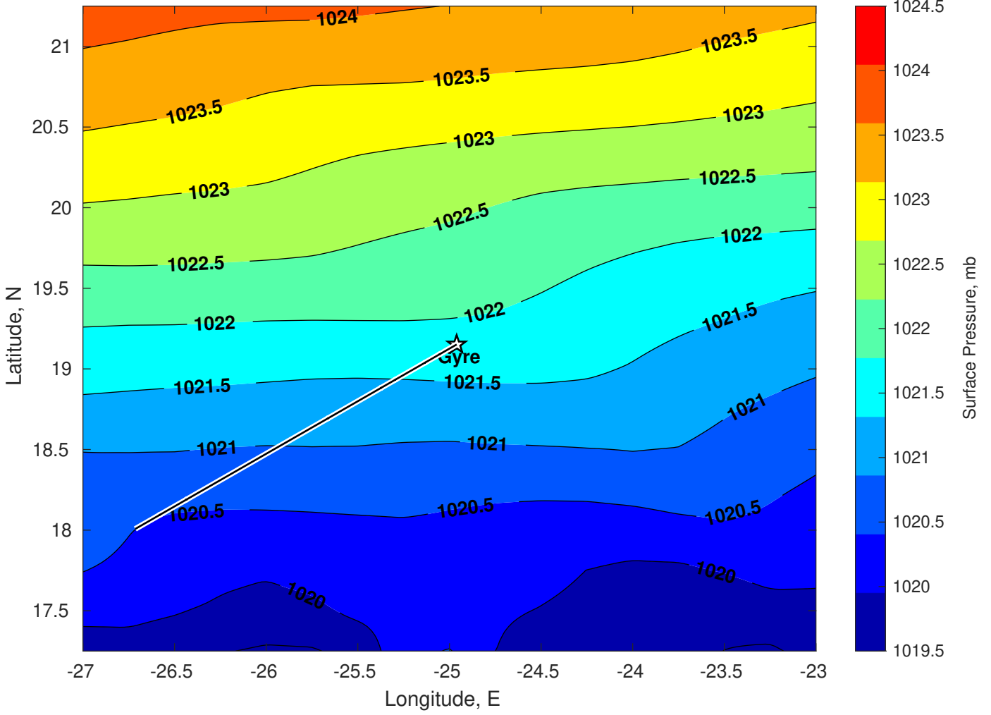
Surface Pressure (mb) for Gyre at 30-Jan-2025 00:00:00
