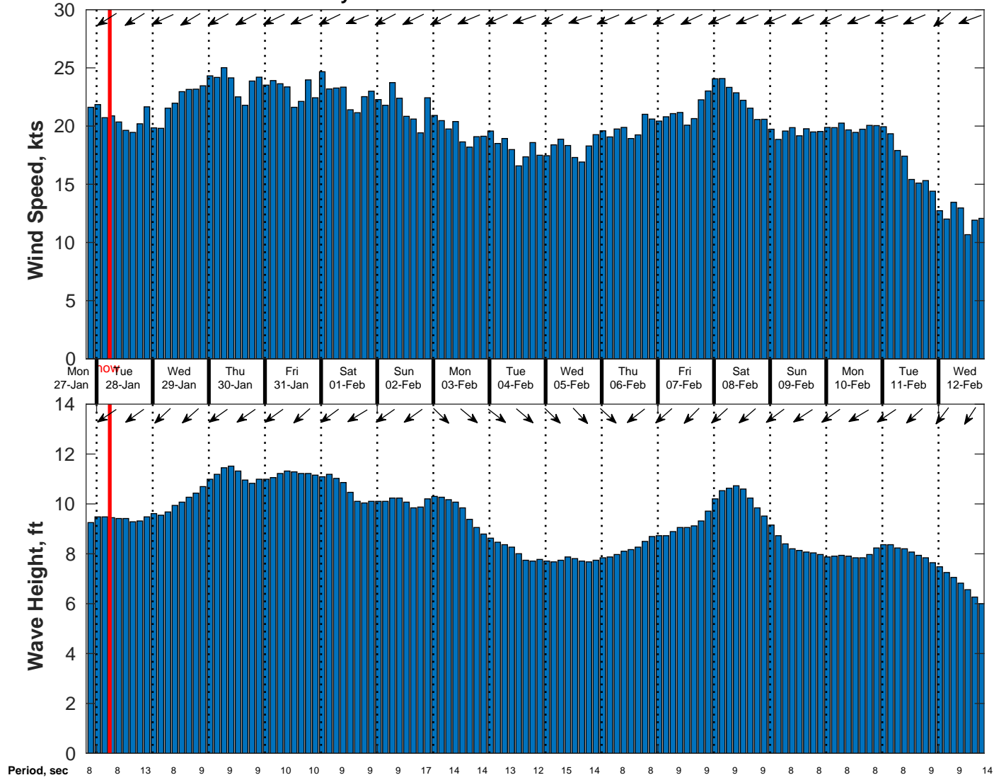
Wind & Wave Forecast for Gyre from 27-Jan-2025 20:00:00 to 12-Feb-2025 20:00:00
