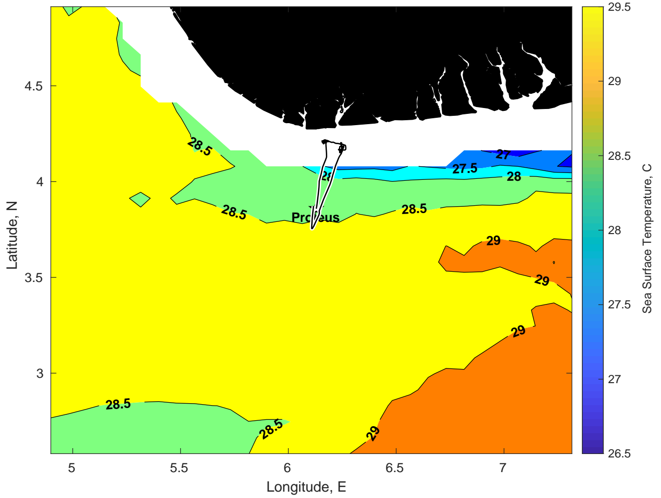
SST for Proteus at 27-Jan-2025 00:00:00
