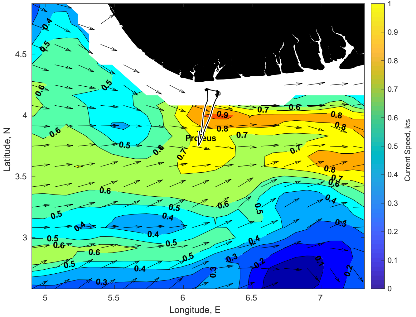
Surface Currents for Proteus at 27-Jan-2025 00:00:00
