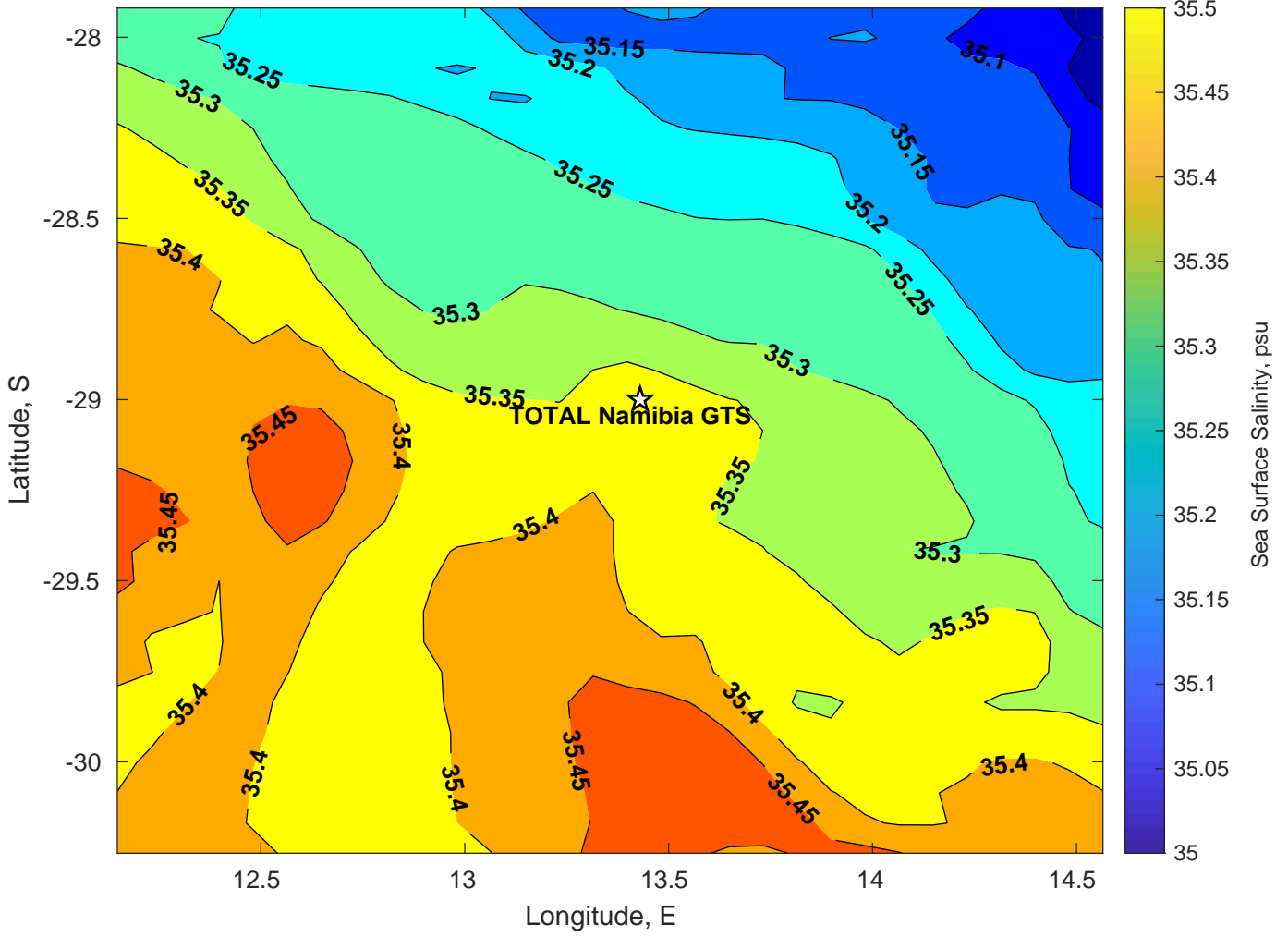
Surface Salinity for TOTAL Namibia GTS at 27-Jan-2025 00:00:00
