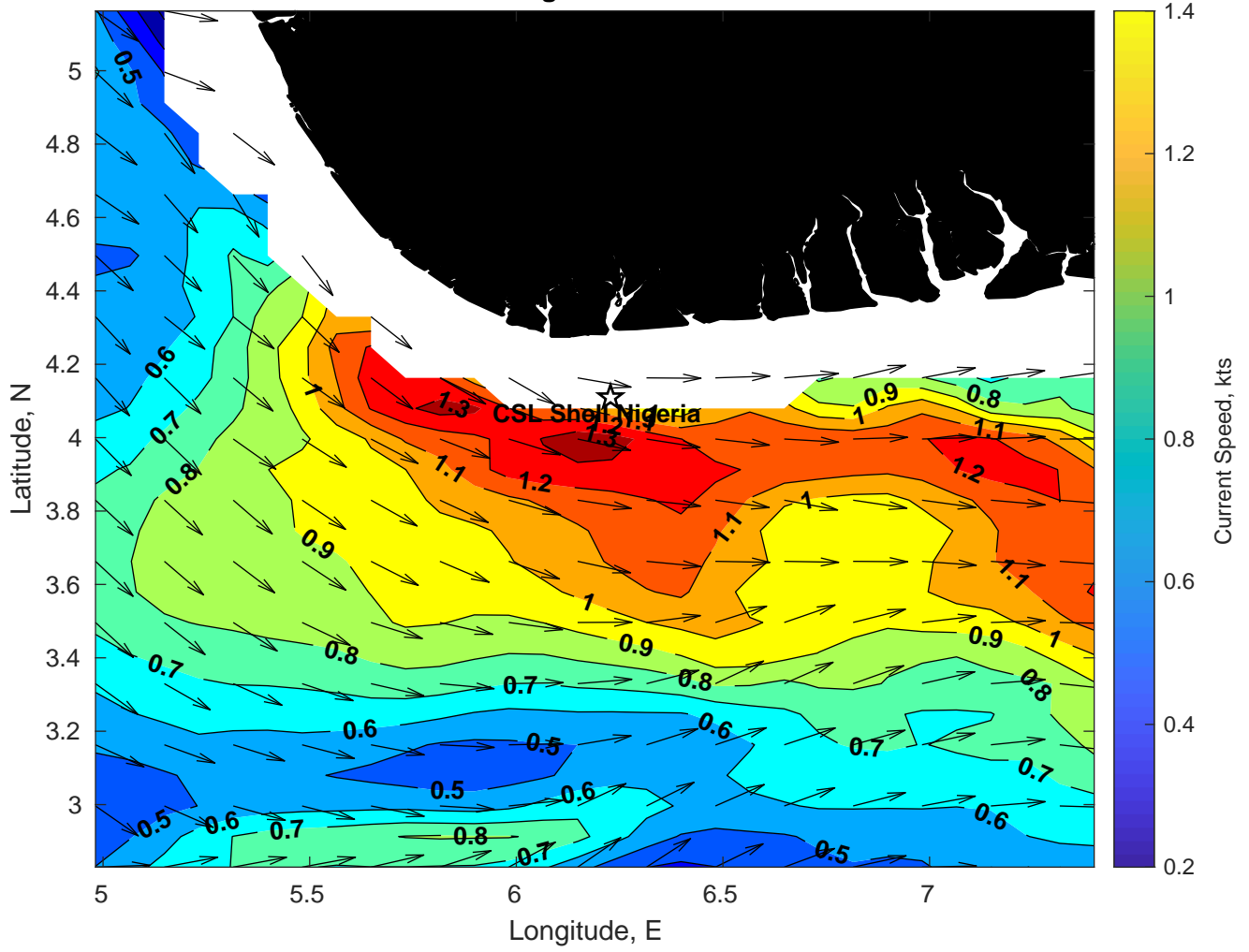
Surface Currents for CSL Shell Nigeria at 28-Jan-2025 00:00:00
