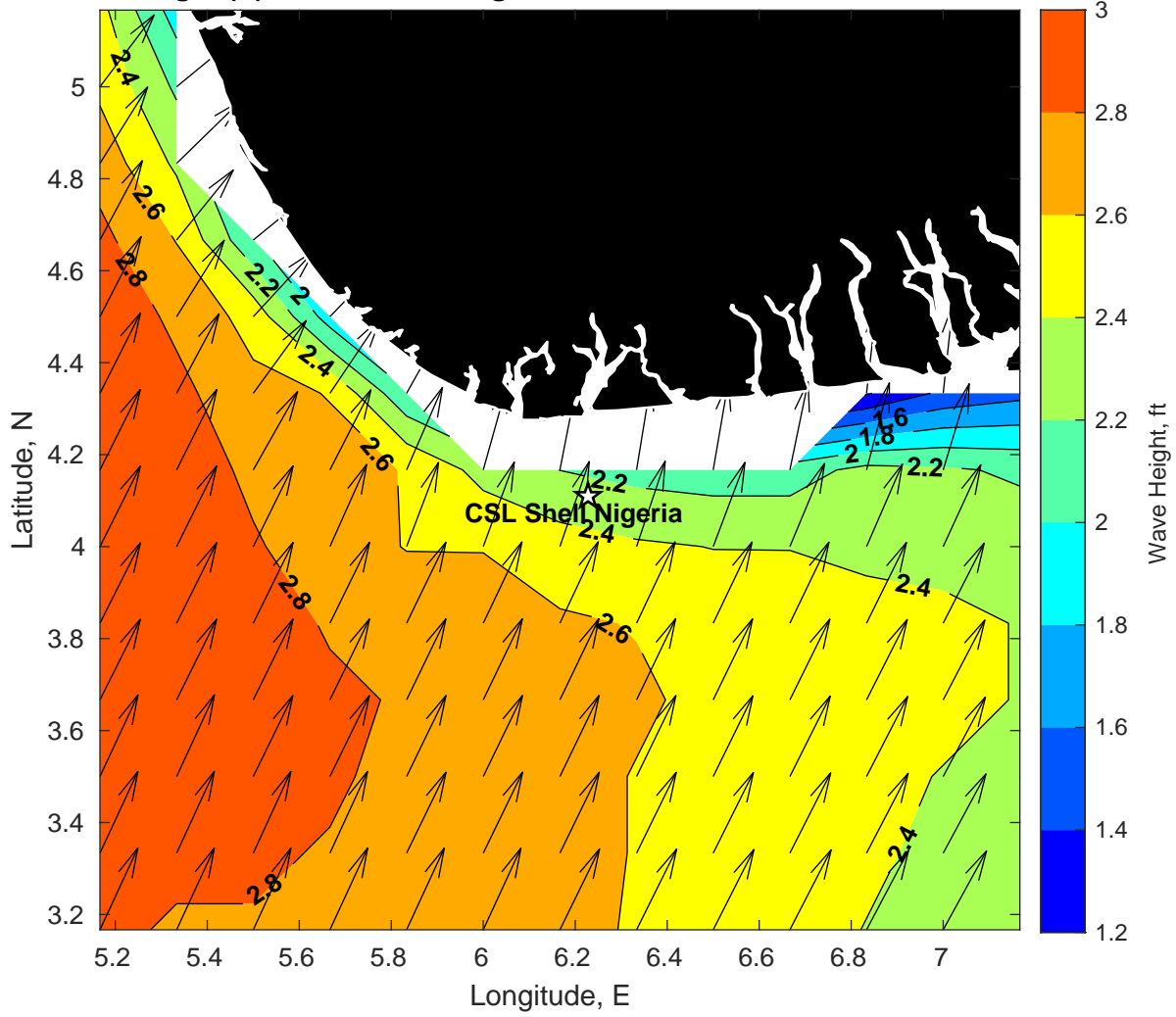
Wave Height (ft) for CSL Shell Nigeria at 29-Jan-2025 09:00:00
