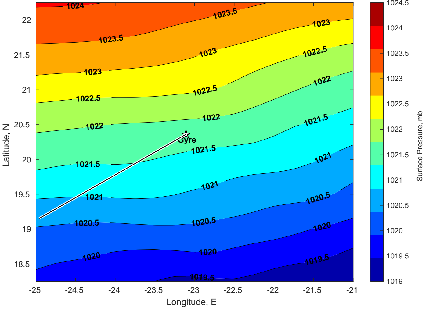
Surface Pressure (mb) for Gyre at 29-Jan-2025 00:00:00
