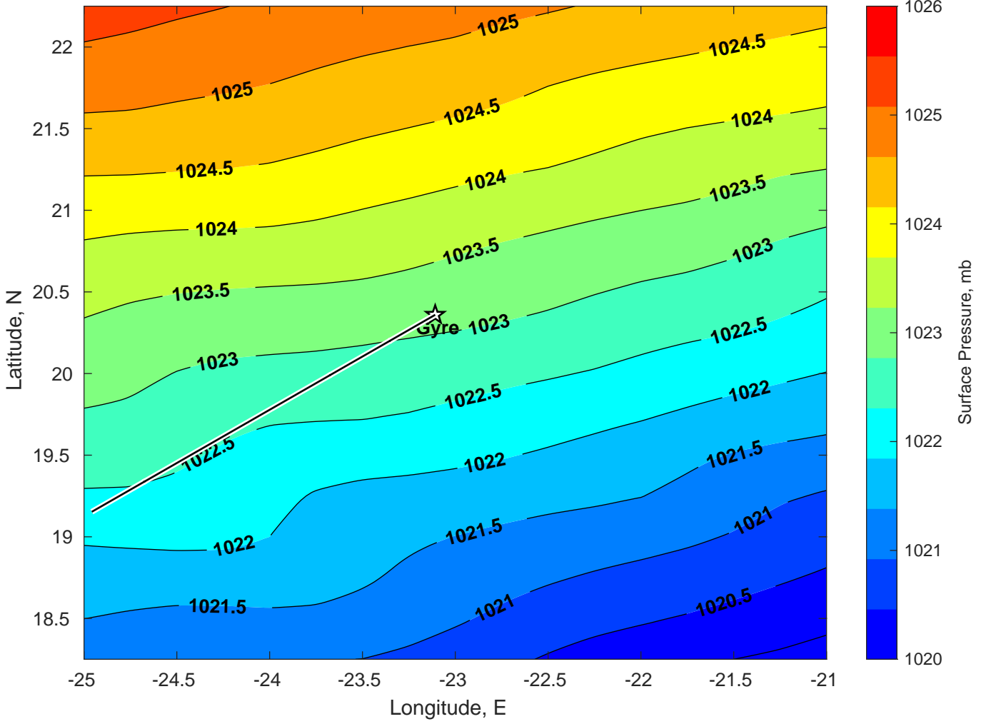
Surface Pressure (mb) for Gyre at 30-Jan-2025 00:00:00
