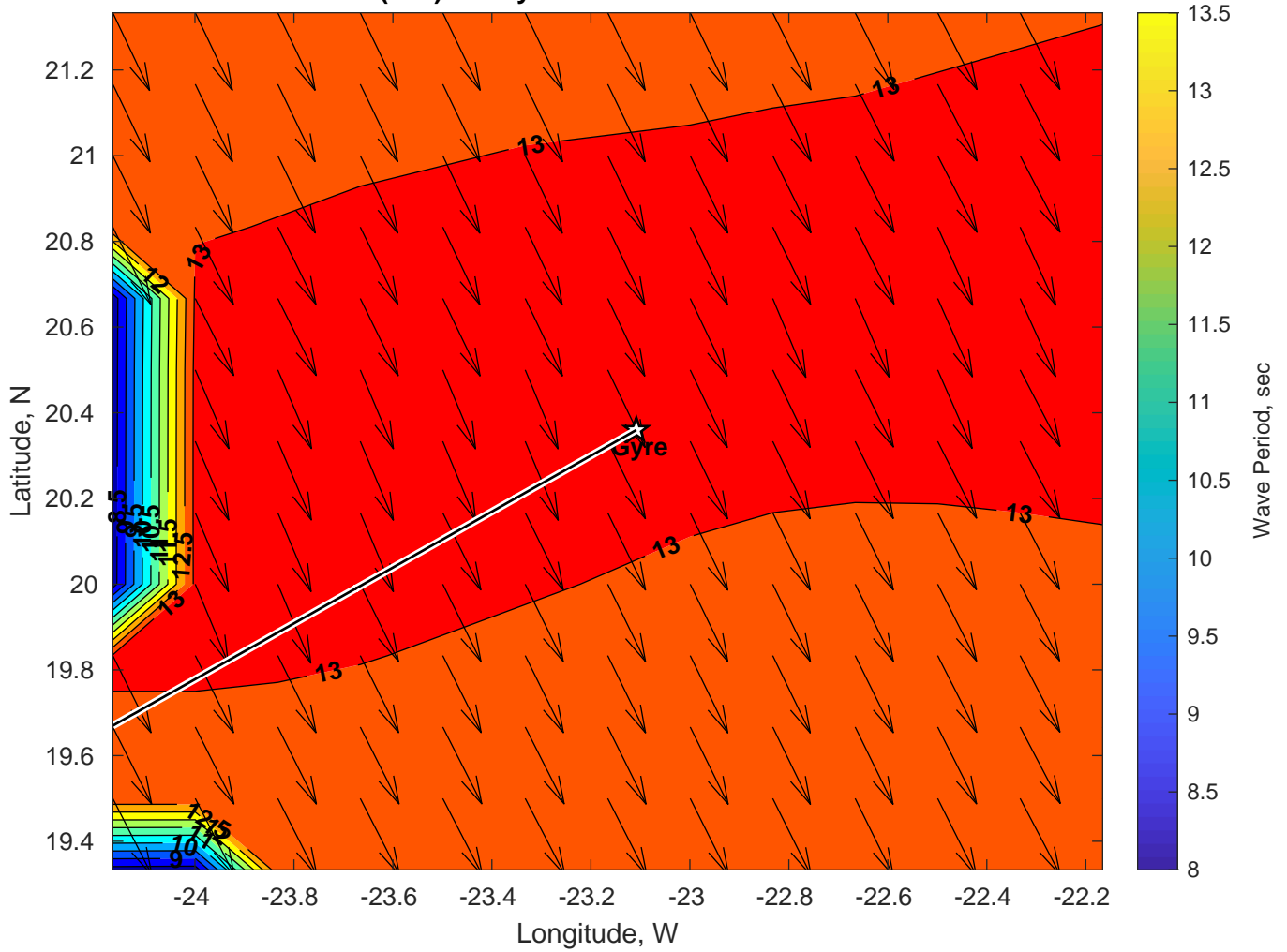
Wave Period (sec) for Gyre at 29-Jan-2025 09:00:00
