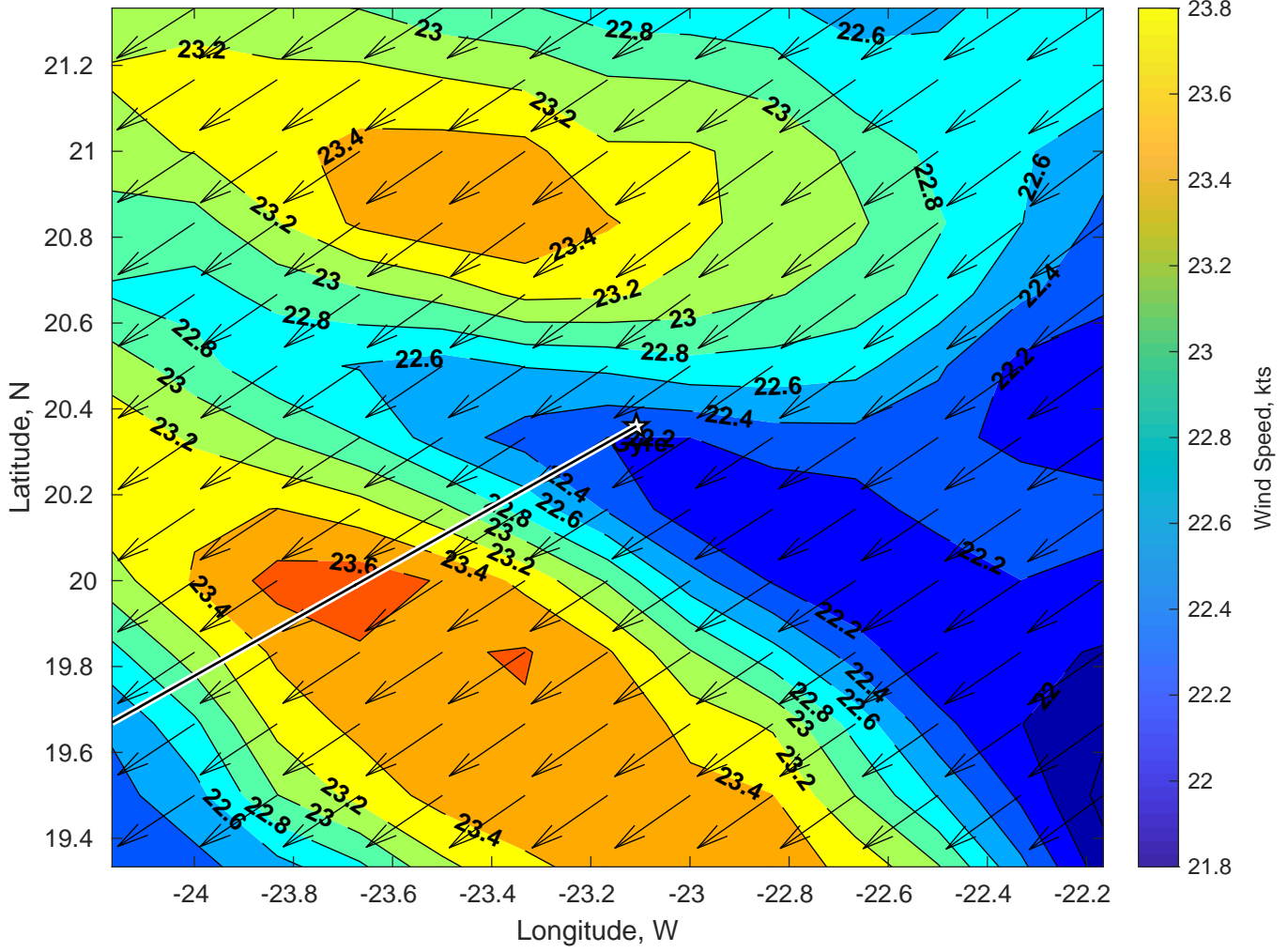
Winds (kts) for Gyre at 29-Jan-2025 09:00:00
