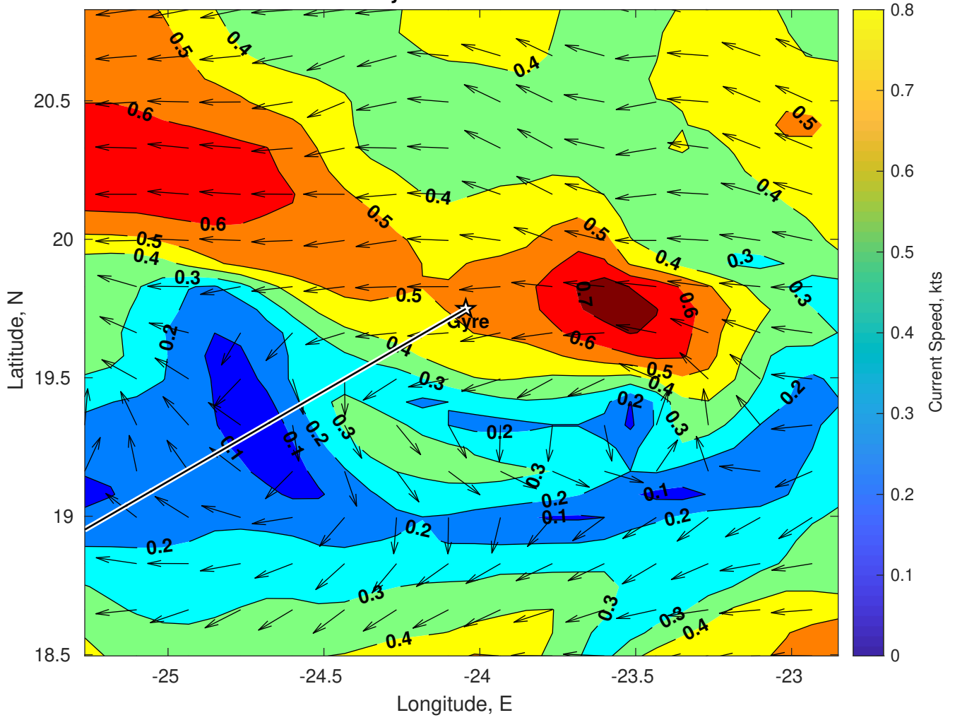
Surface Currents for Gyre at 28-Jan-2025 00:00:00
