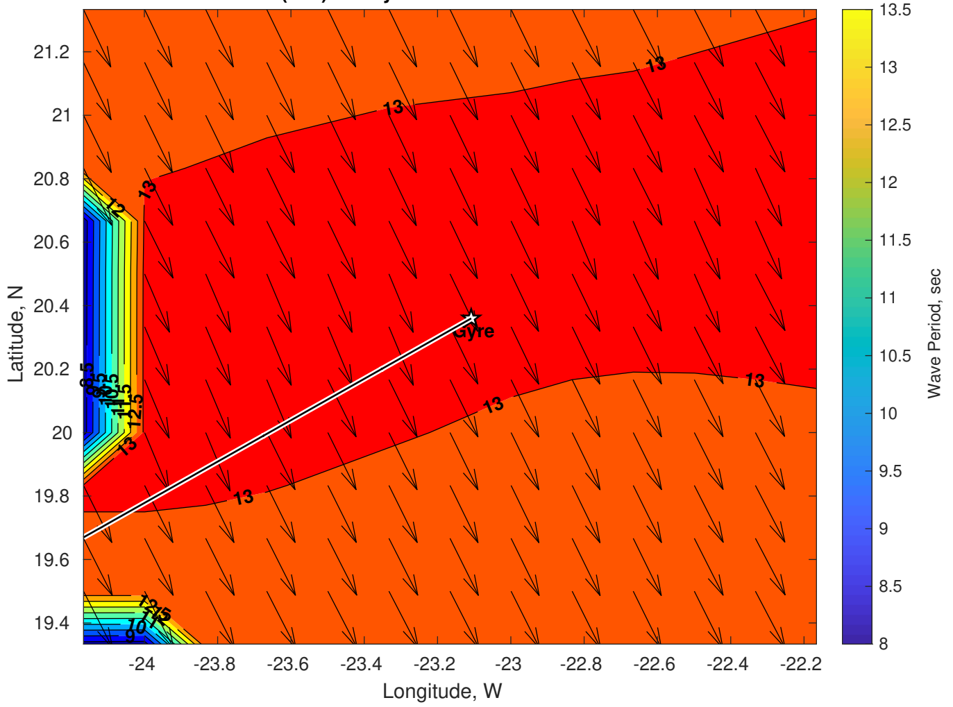
Wave Period (sec) for Gyre at 29-Jan-2025 09:00:00
