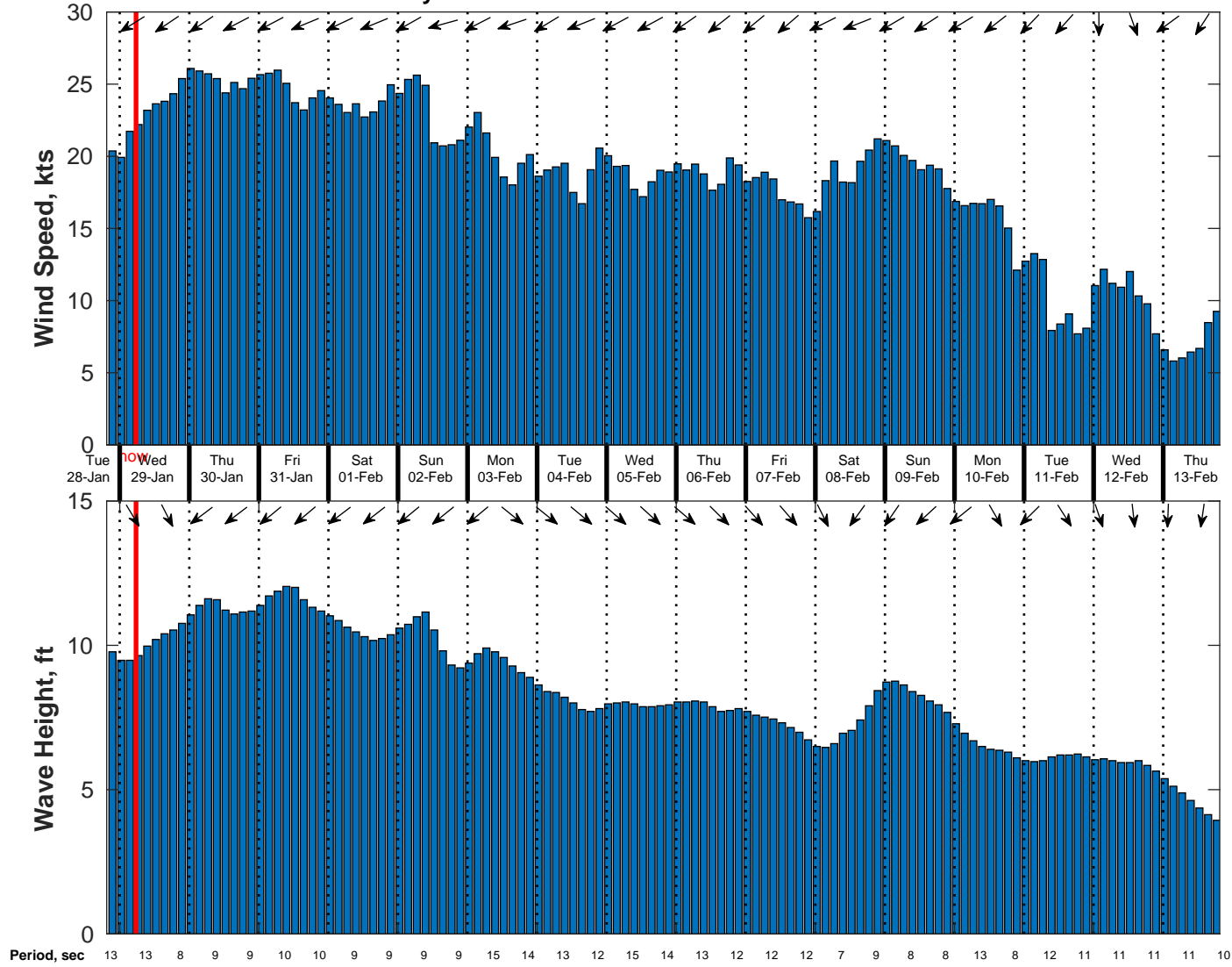
Wind & Wave Forecast for Gyre from 28-Jan-2025 20:00:00 to 13-Feb-2025 20:00:00
