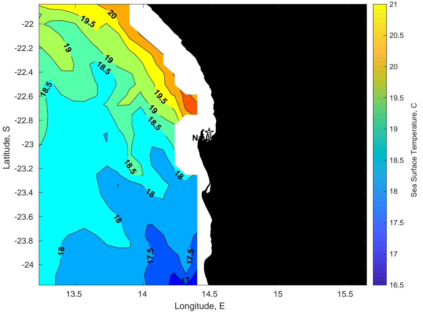
SST for Nautilus at 28-Jan-2025 00:00:00
