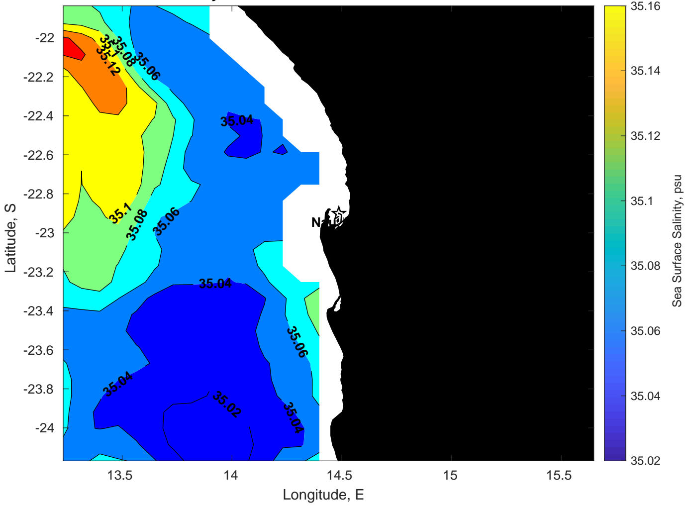
Surface Salinity for Nautilus at 28-Jan-2025 00:00:00
