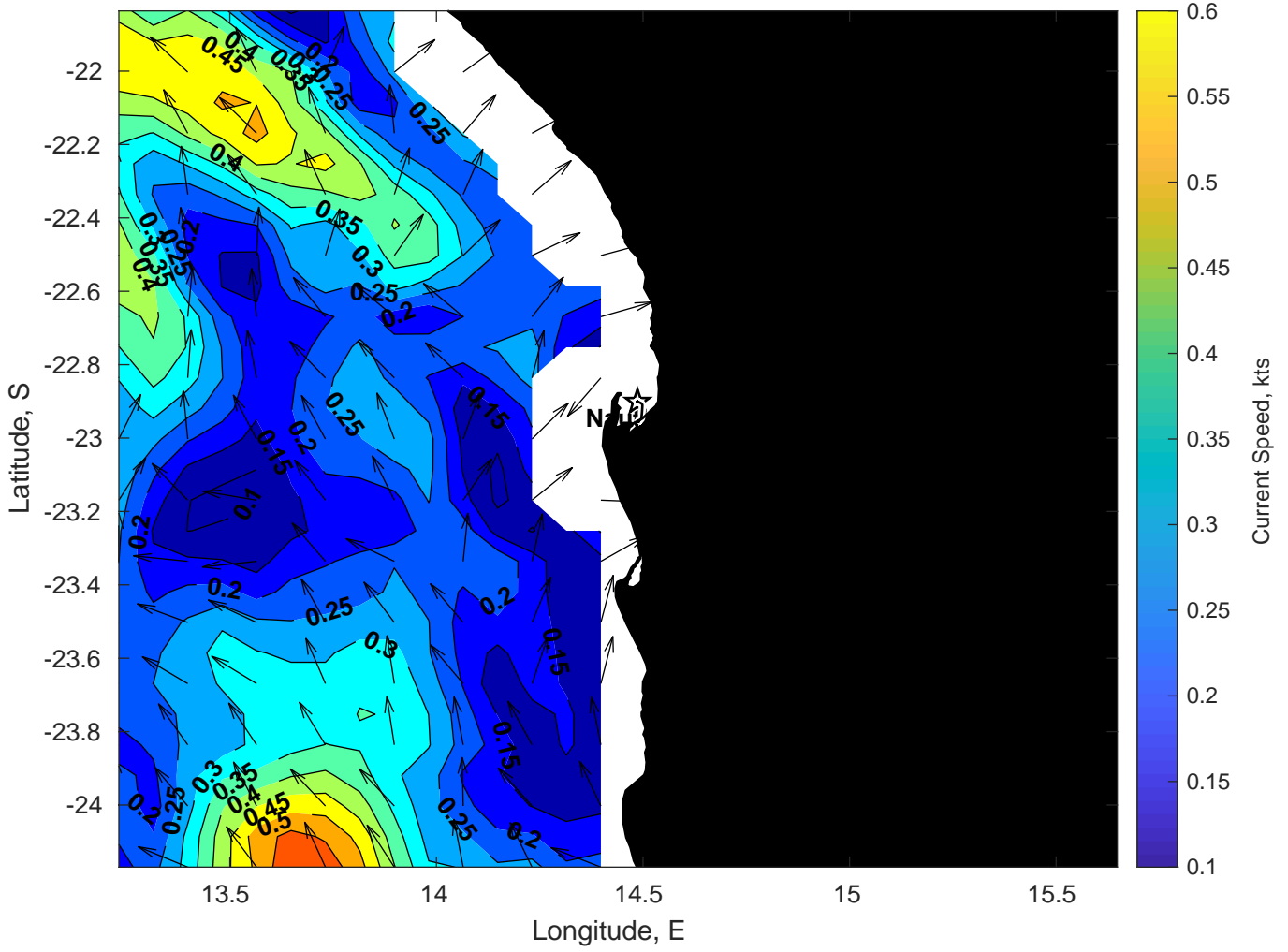
Surface Currents for Nautilus at 28-Jan-2025 00:00:00
