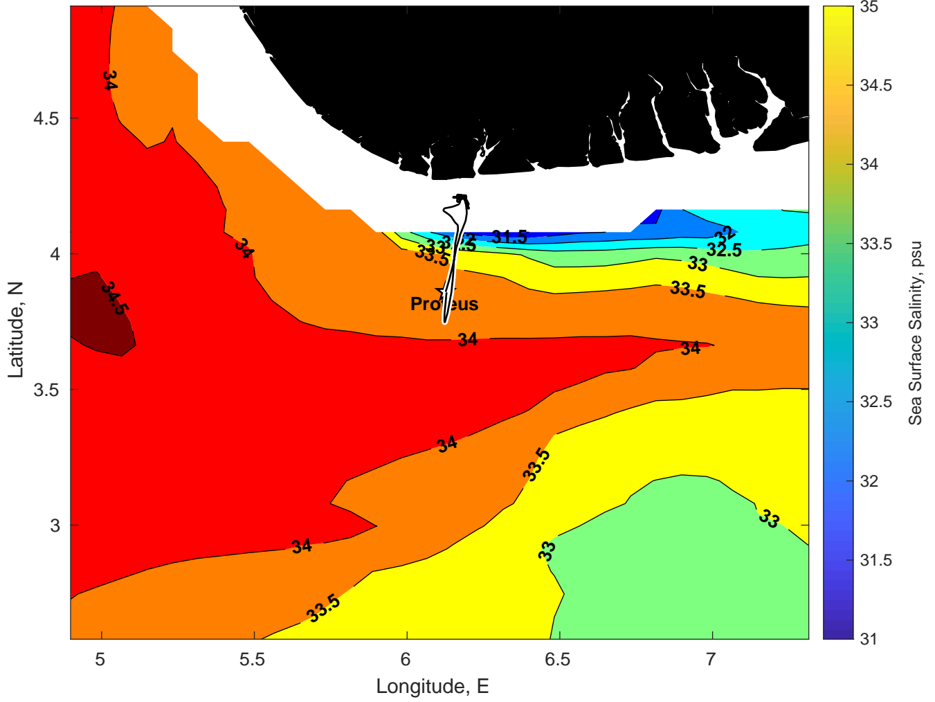
Surface Salinity for Proteus at 28-Jan-2025 00:00:00
